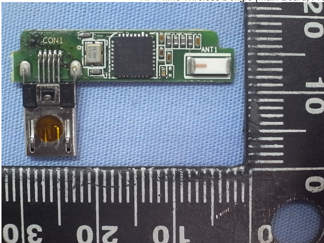
HP Prime Wireless Dongle (Main Board, Front View)
