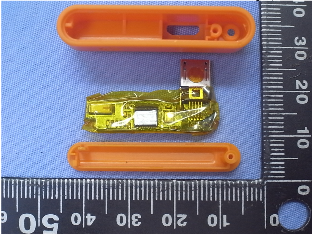
HP Prime Wireless Dongle (Removed Covers)
