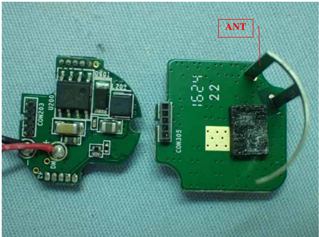
Figure 5 Internal View
