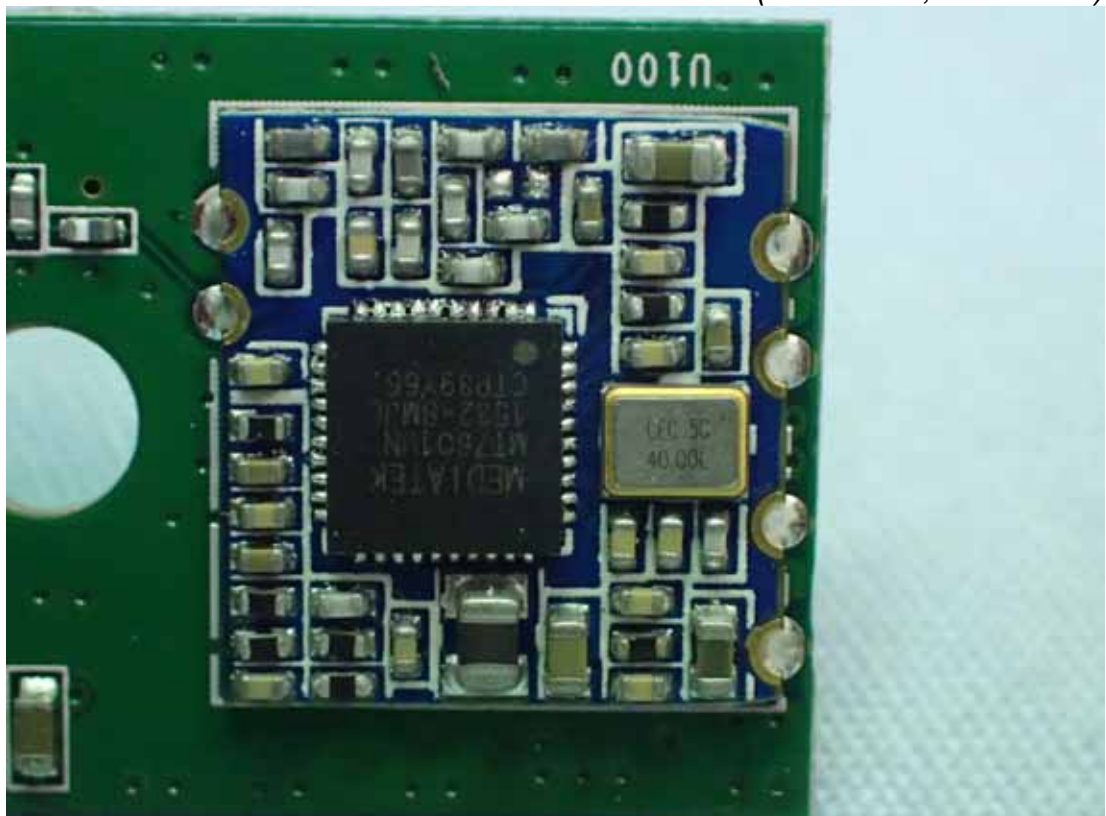
Figure 8 Internal View (RF Module, Front View)
