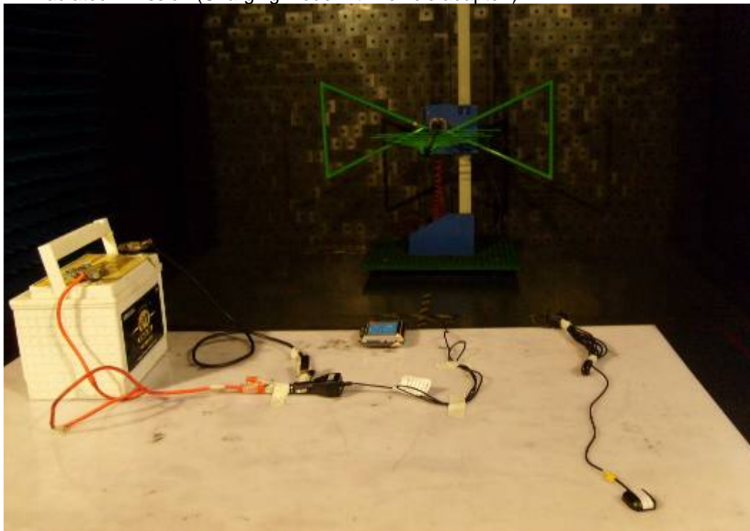
Radiated Emission (Charging mode with vehicle adapter )
