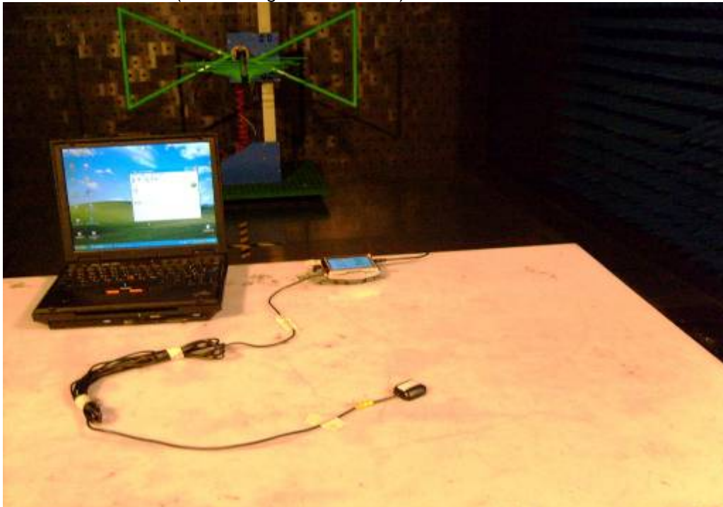
Radiated Emission (Connecting with PC mode)
