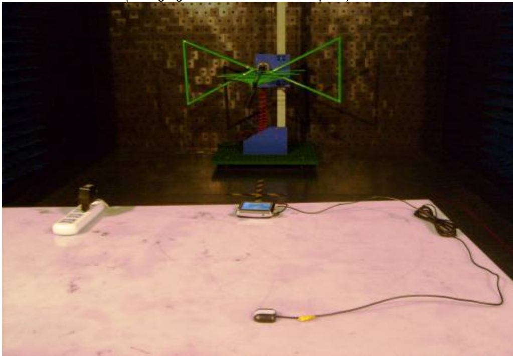
Radiated Emission (Charging mode with AC/DC adapter )
