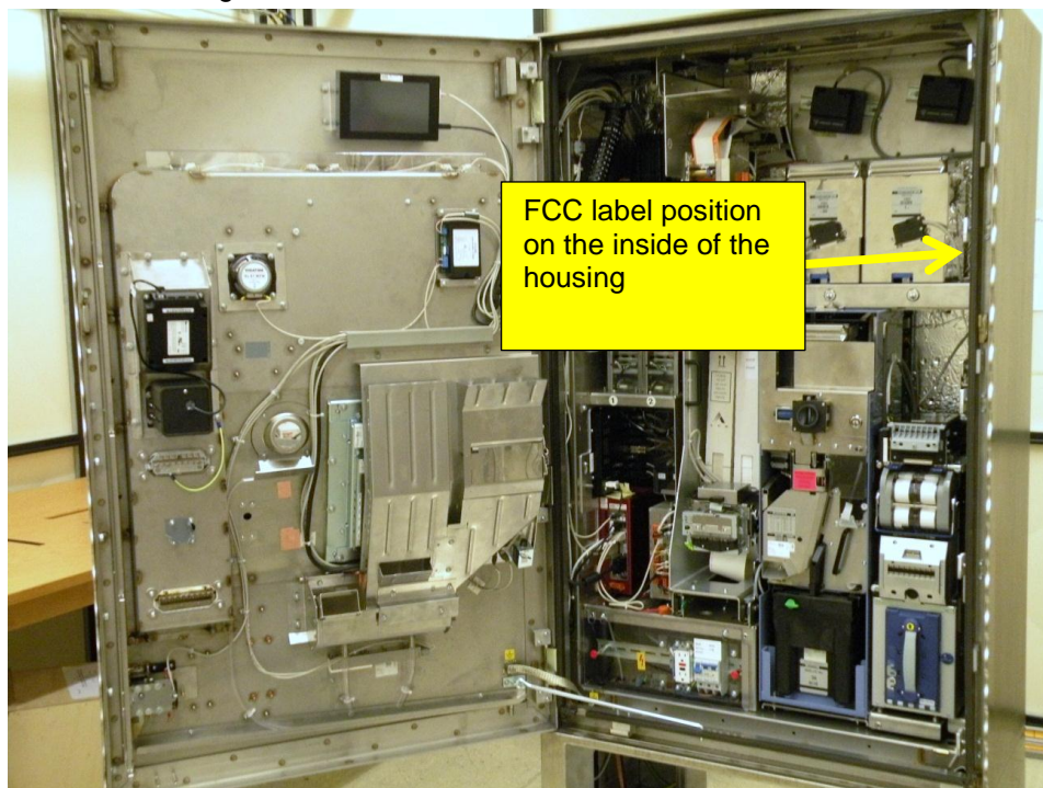
Inside view of ticket vending machine and FCC label location
