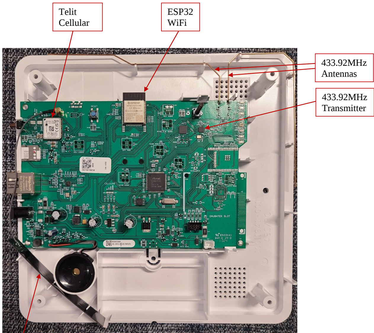
PCBA in Enclosure
