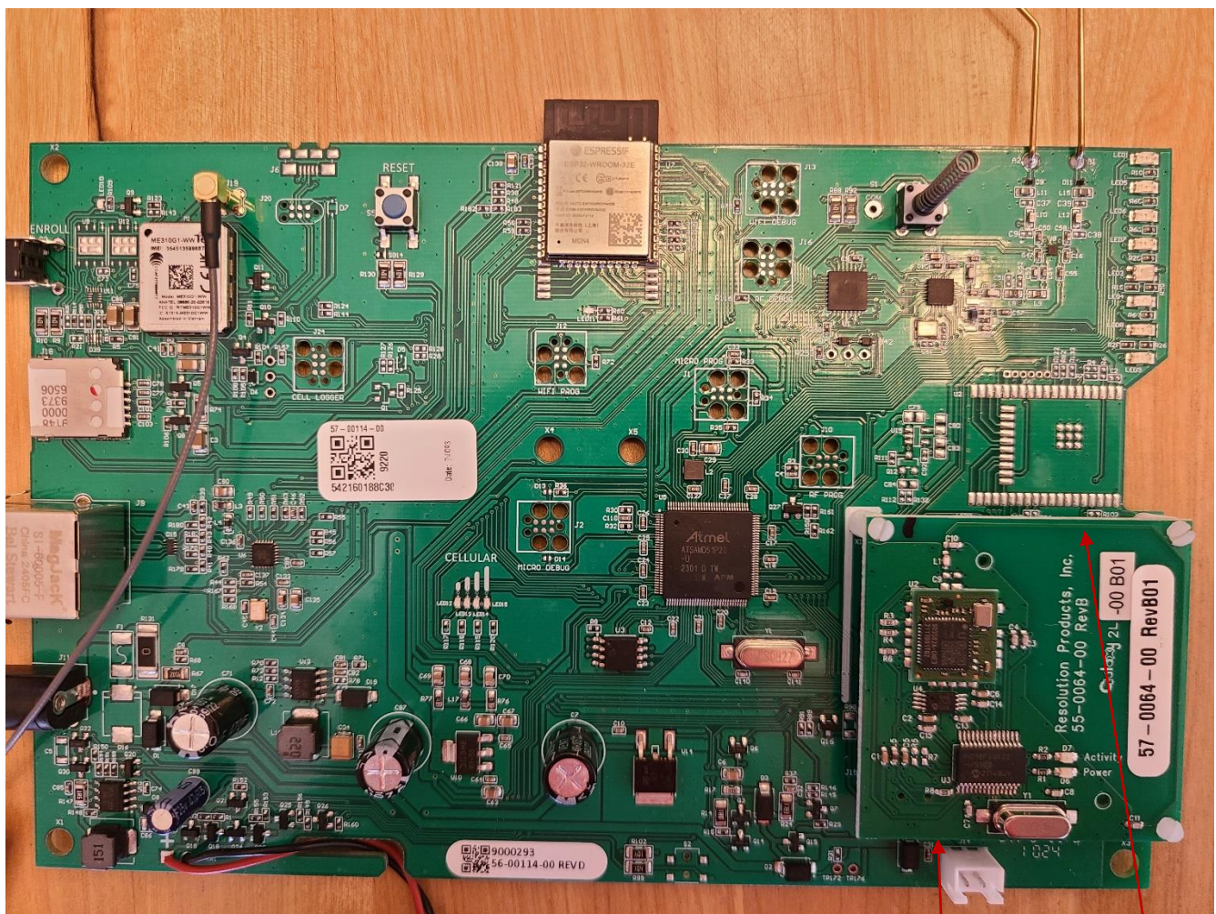
PCBA Top, with optional Zwave Module installed
