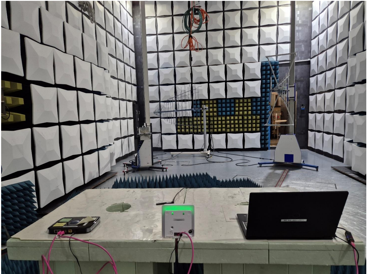
Photo 3: Test setup for radiated measurements, unintentional radiator (semi-anechoic chamber 1 GHz – 18 GHz)
