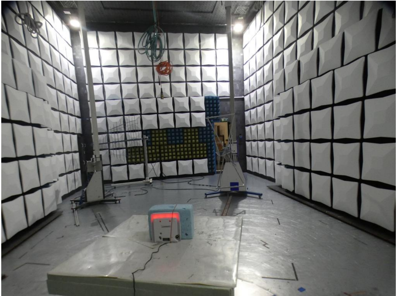
Photo 5: Test setup for radiated measurements, intentional radiator (semi-anechoic chamber 30 MHz – 1 GHz)
