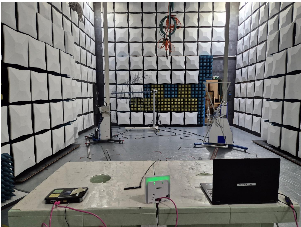
Photo 2: Test setup for radiated measurements, unintentional radiator (semi-anechoic chamber 30 MHz – 1 GHz)
