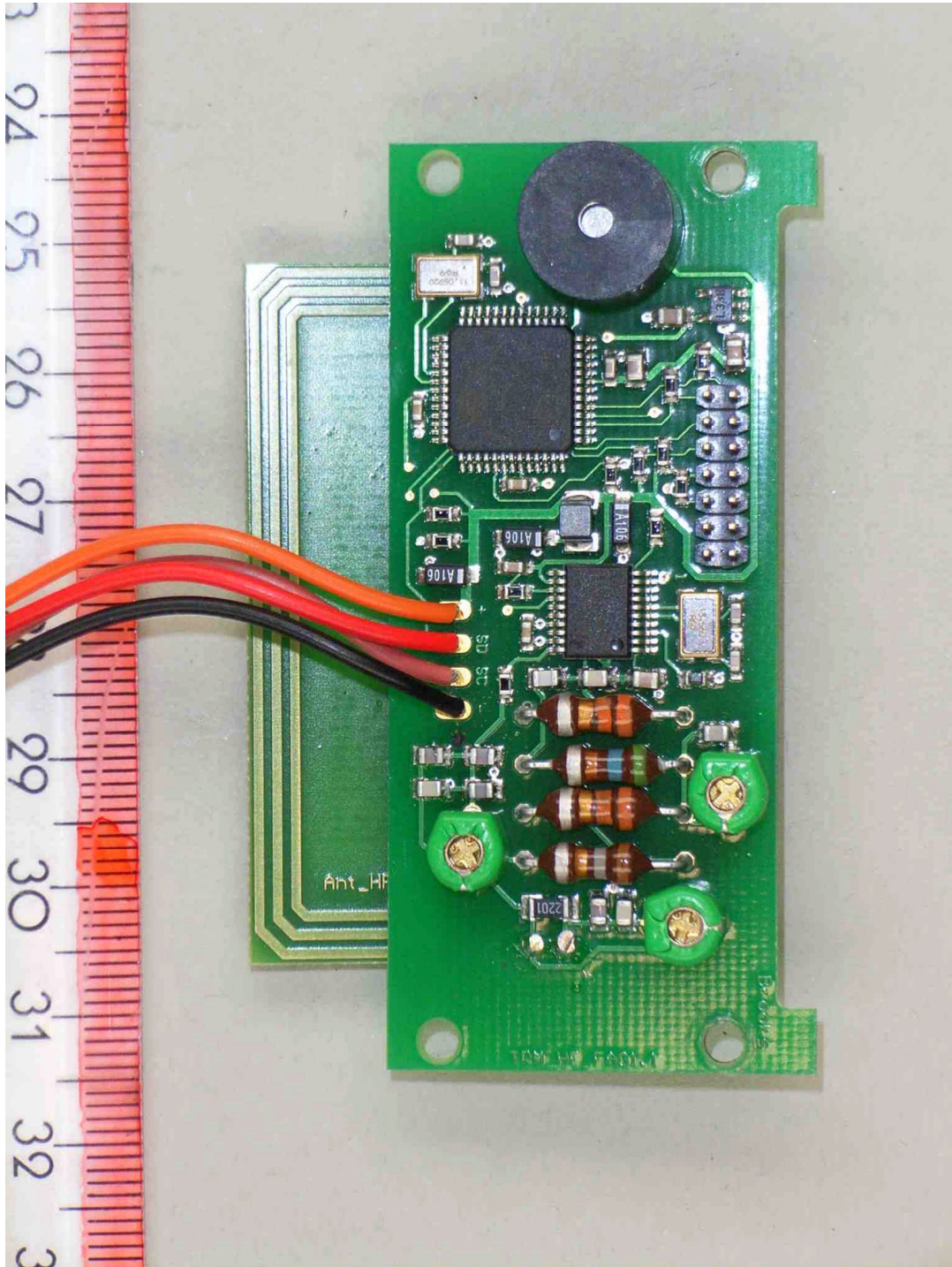
70363eut8.jpg: RF-PCB, top view
