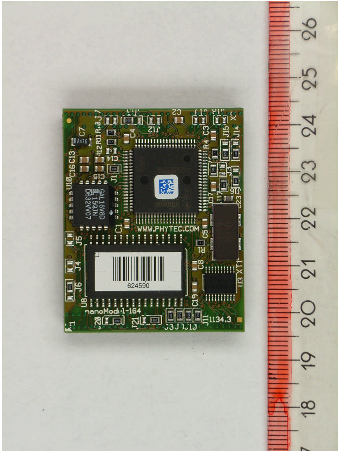
70363eut24.jpg: sub board, top view
