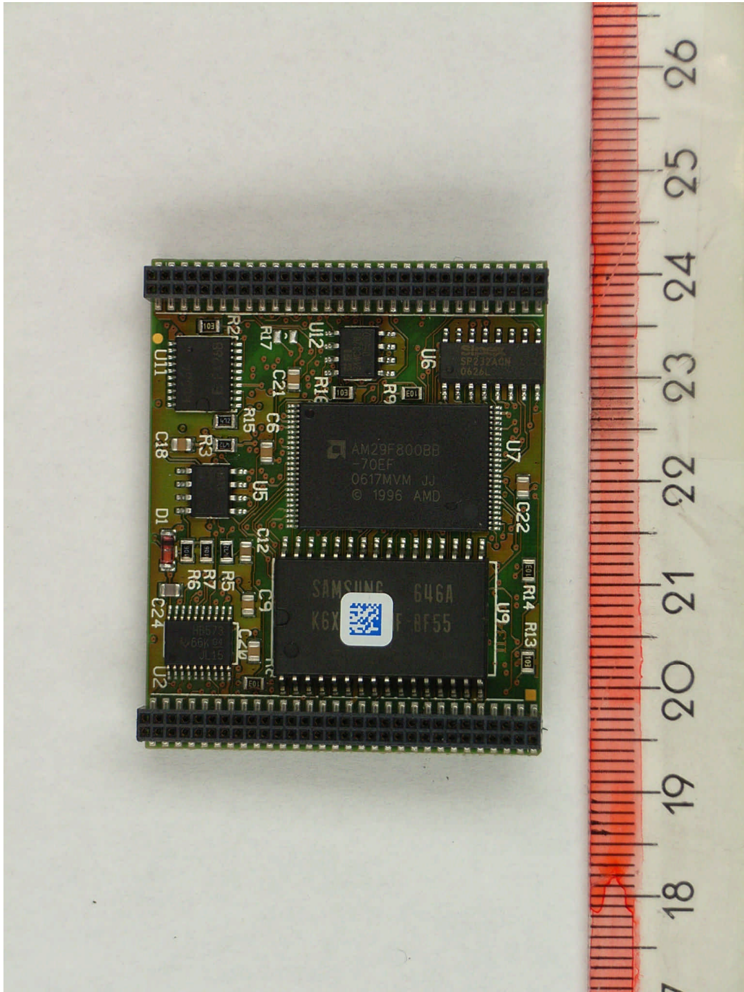
70363eut25.jpg: sub board, bottom view
