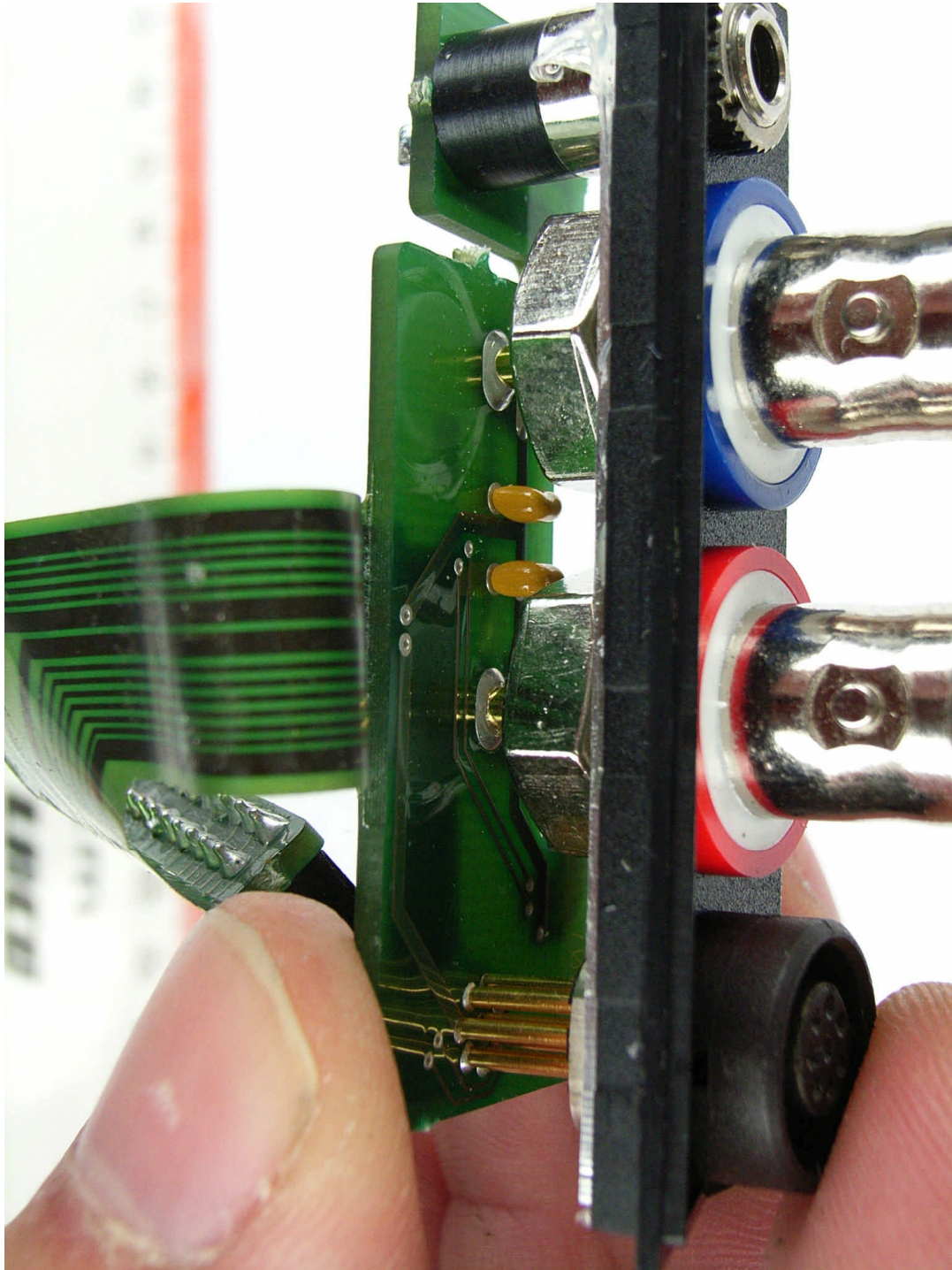
70363eut32.jpg: connection board, bottom view detail
