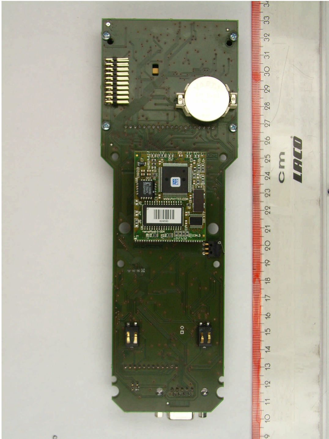
70363eut21.jpg: Main-PCB, bottom view
