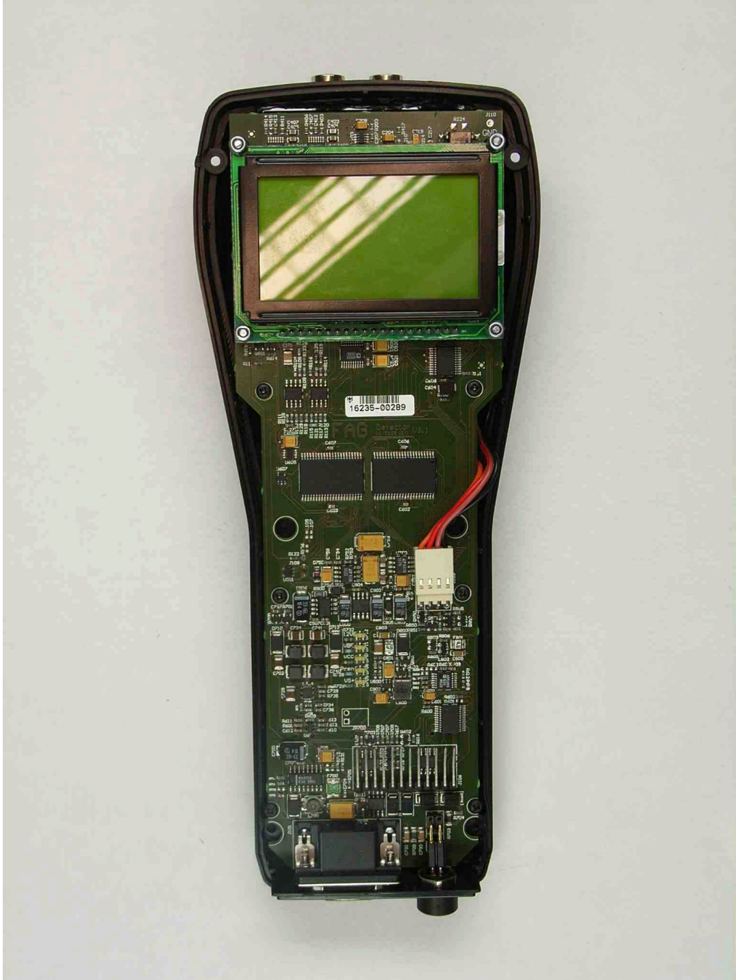
70363eut9.jpg: Main-PCB, top view
