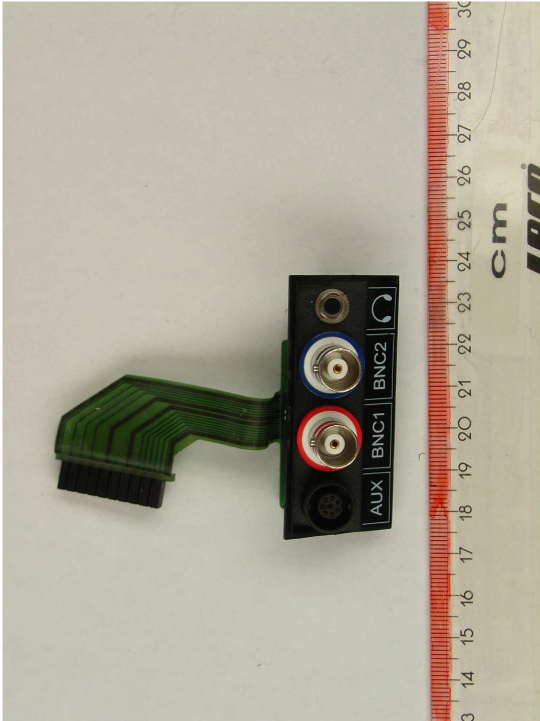
70363eut31.jpg: connection board, bottom view
