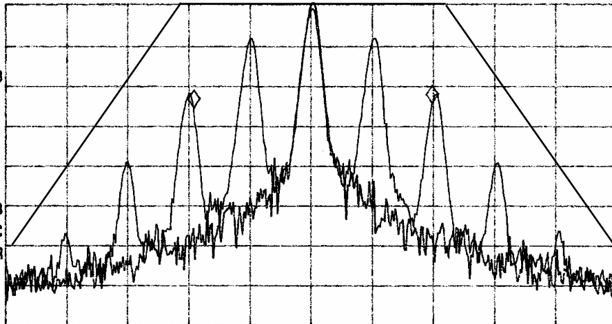
Figure eight Occupied Band Width, Narrow band, no squelch tone
