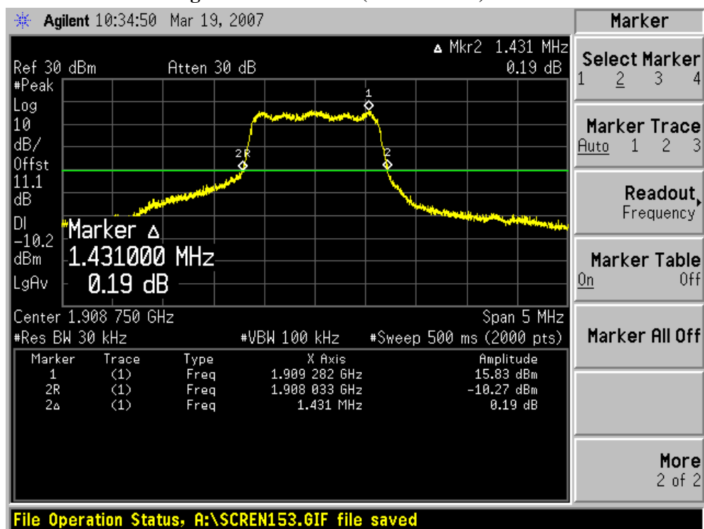
Figure Channel 1175 (1908.75MHz)
