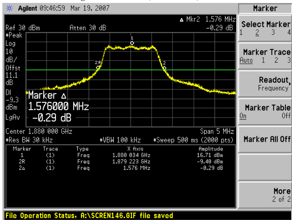
Figure Channel 600 (1880.00MHz)
