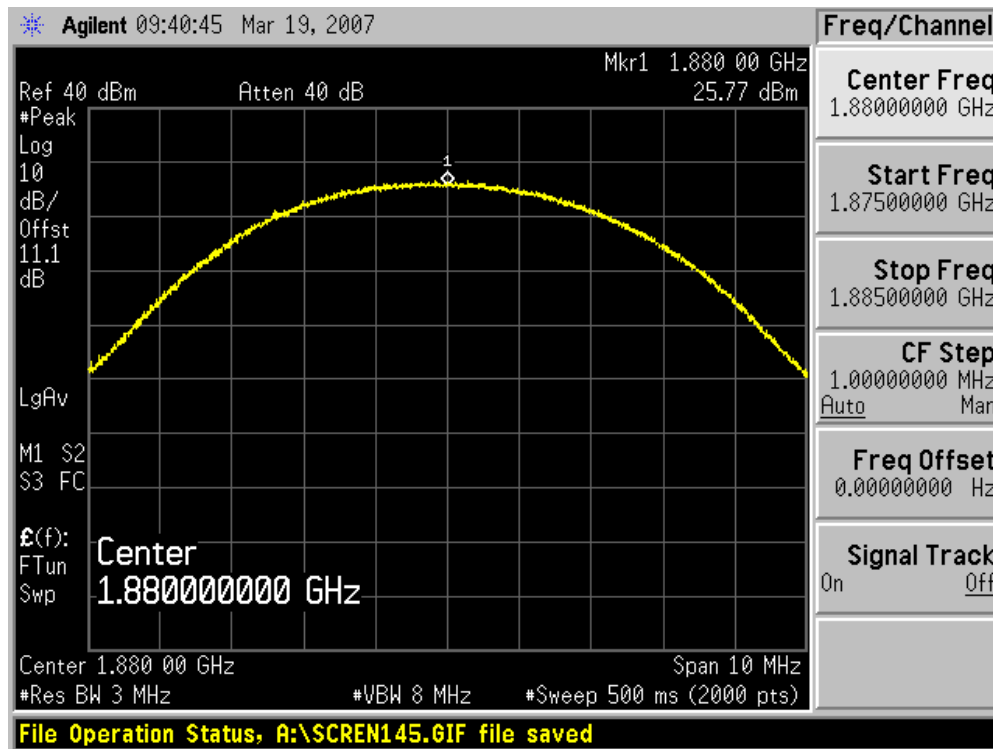
Figure Channel 600 (1880.00MHz)
