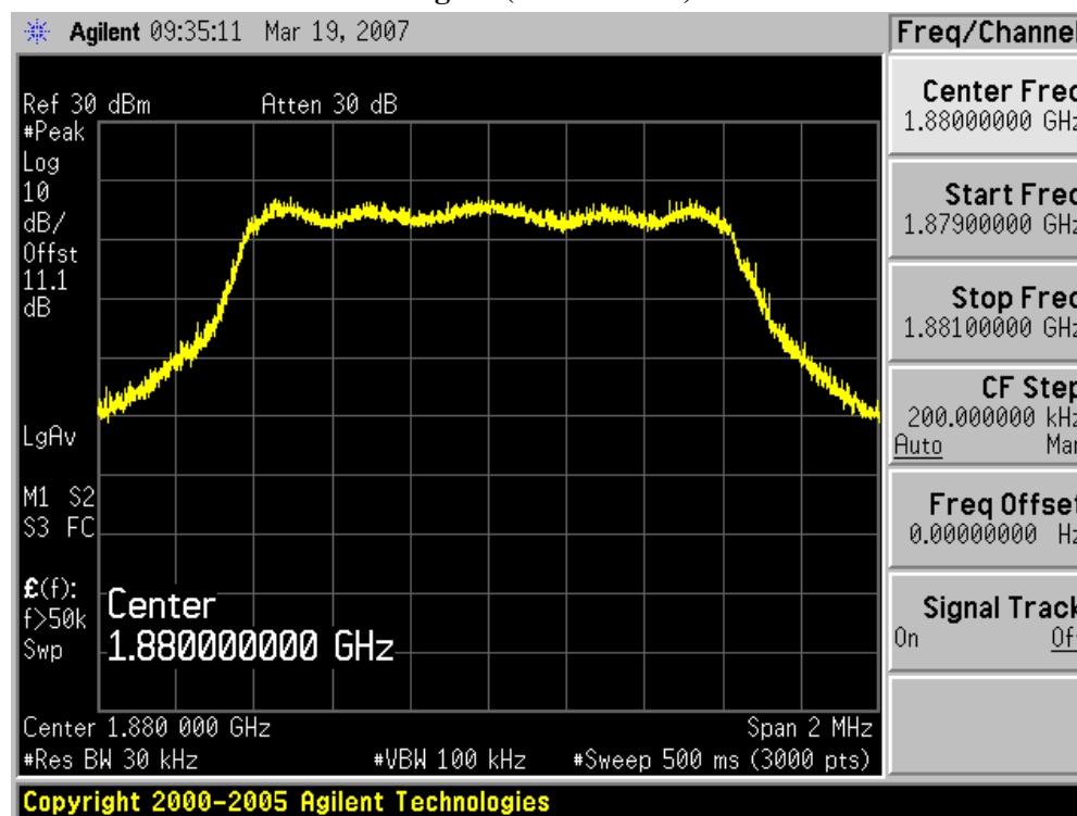
Figure (CDMA 1900)
