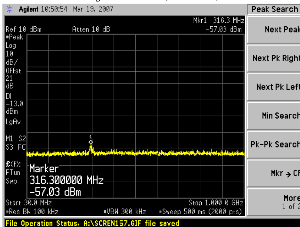
Figure Channel 600 (1880.00MHz)
