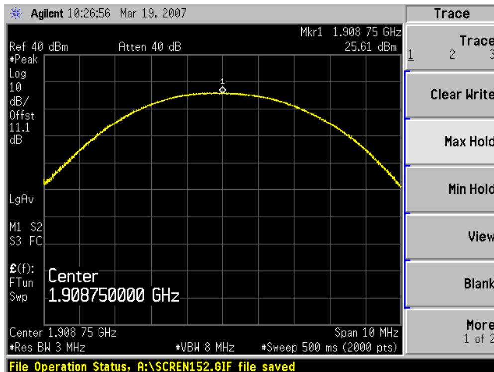
Figure Channel 1175 (1908.75MHz)
