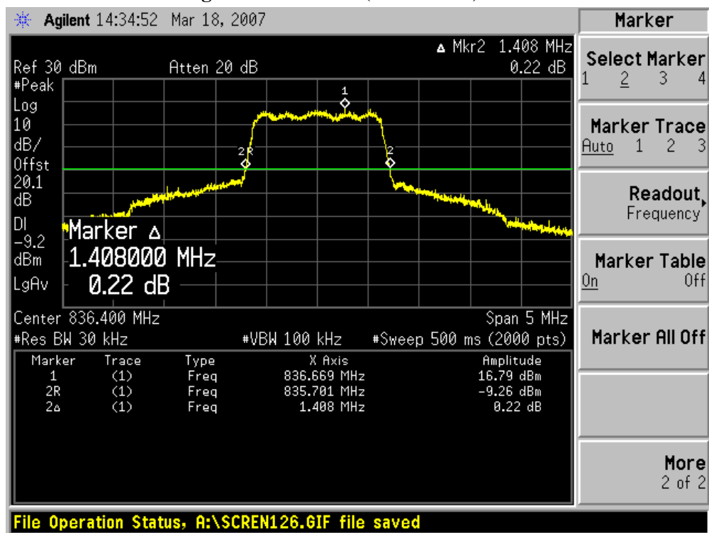
Figure Channel 380 (836.40MHz)
