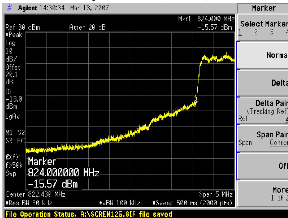
Figure Channel 1014 (824.73MHz)
