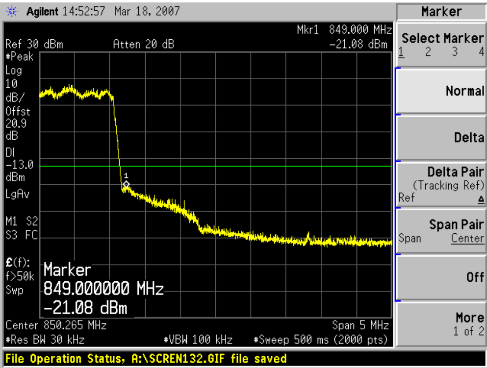
Figure Channel 773 (848.19MHz)
