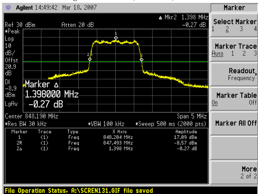
Figure Channel 773 (848.19MHz)
