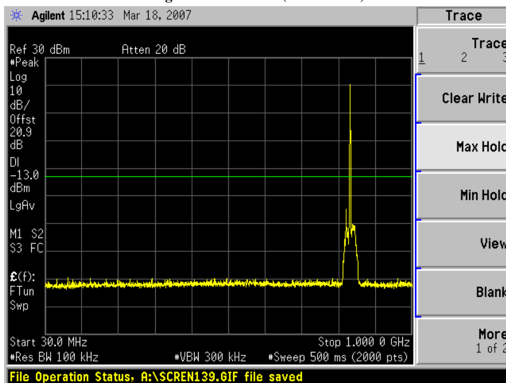
Figure Channel 380 (836.40MHz)
