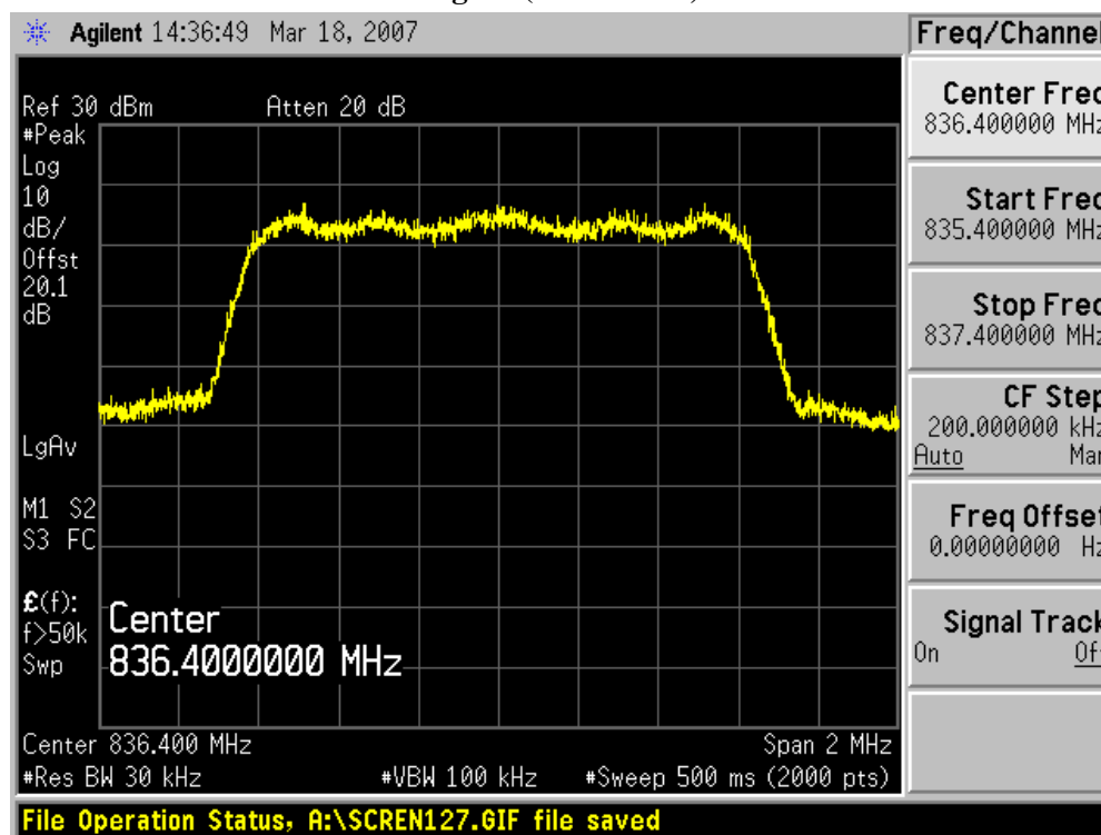
Figure (CDMA 850)
