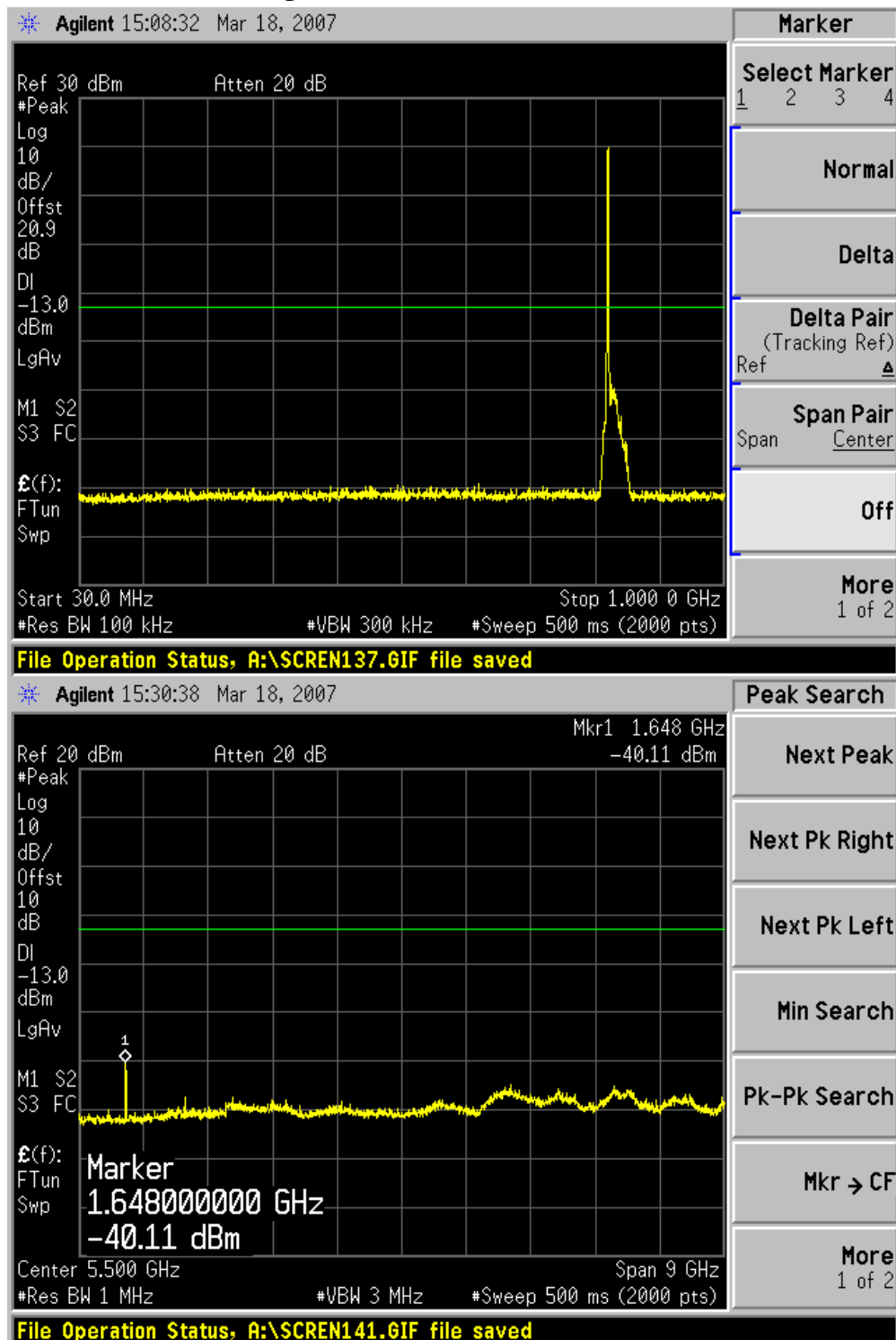
Figure Channel 1014 (824.73MHz)
