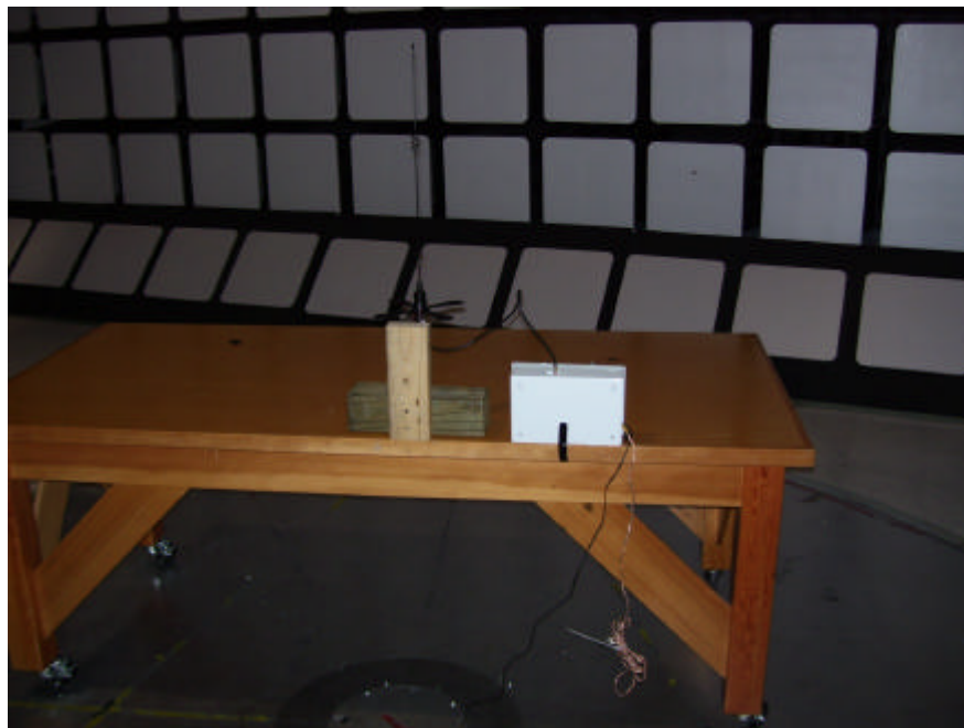
Figure 16 - Radiated Emissions, Whip Antenna
