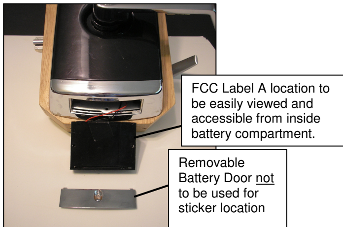
Sticker Location for Wireless Cylindrical Lockset (WCL)
