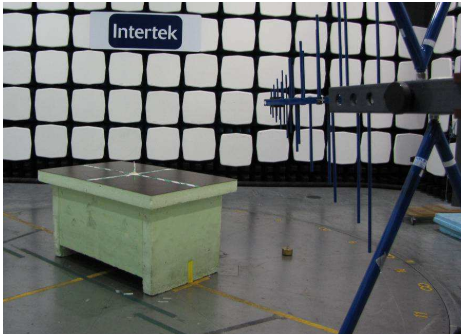
Radiated spurious emission 30-1000 MHz
