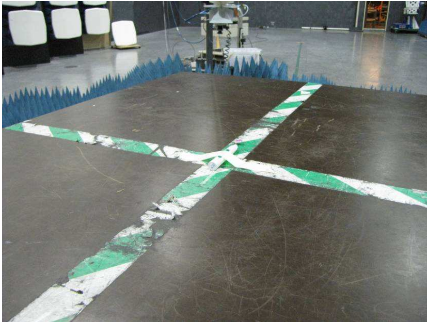
Radiated spurious emission above 1 GHZ, photo Big Chamber (worst case position)
