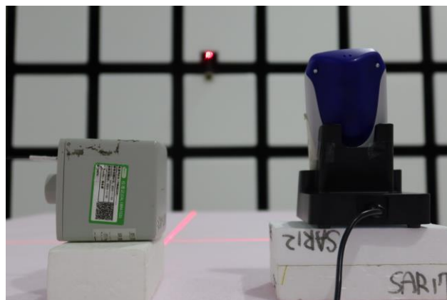
Right Side @ 15cm separation distance
