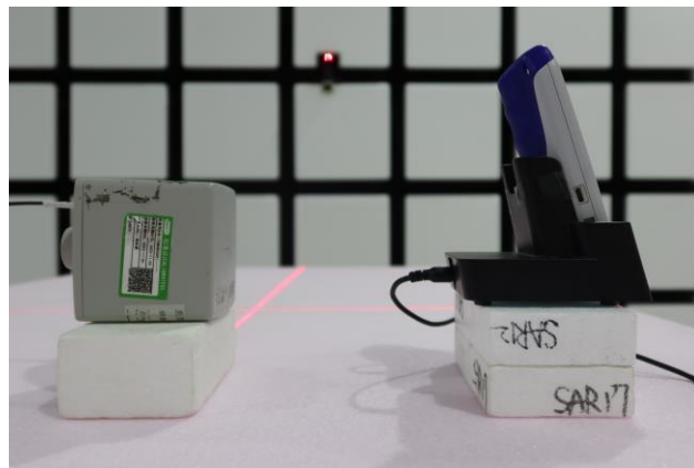
Back @ 20cm separation distance
