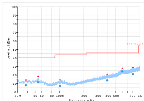
Radiated Spurious Emission (802.11a, ch165, 30 MHz-1 GHz)
