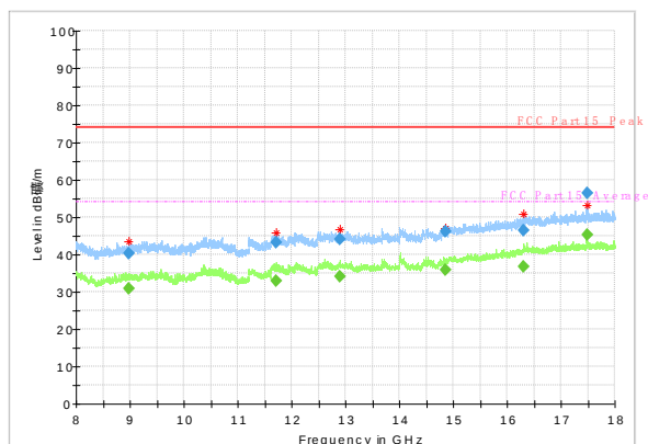
Radiated Spurious Emission (802.11a, ch165, 8GHz-18GHz)
