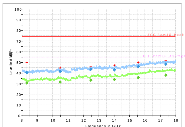
Radiated Spurious Emission (802.11a, ch40, 8GHz-18GHz)
