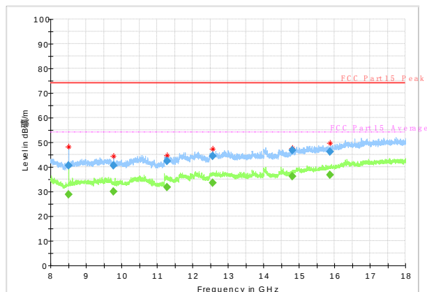
Radiated Spurious Emission (802.11a, ch64, 8GHz-18GHz)
