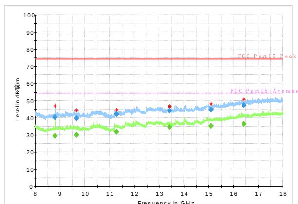
Radiated Spurious Emission (802.11a, ch100, 8GHz-18GHz)
