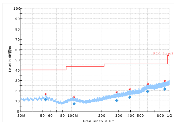
Radiated emission:Ch0, 30MHz~1GHz
