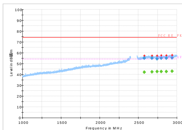
Radiated emission: Ch39, 1GHz~3GHz
