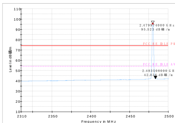
Bandedge:Ch39
