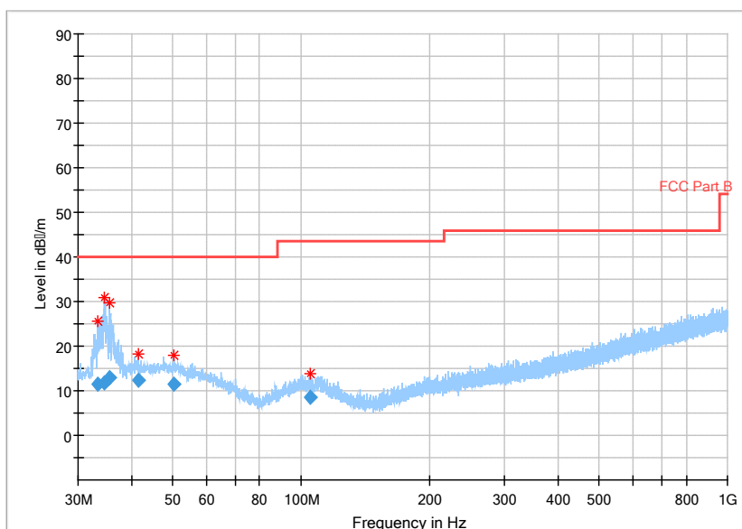
Fig.50 Radiated emission: 8DPSK, Ch78, 30MHz~1GHz
