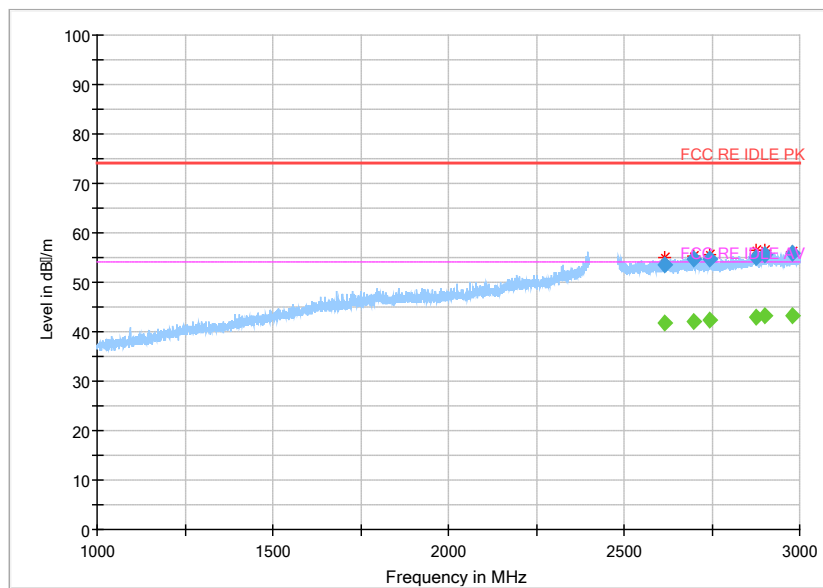
Fig.41 Radiated emission: GFSK, Ch78, 1GHz~3GHz
