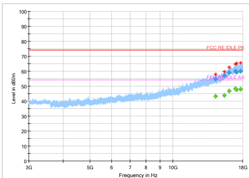
Fig.42 Radiated emission: GFSK, Ch78, 3GHz~18GHz
