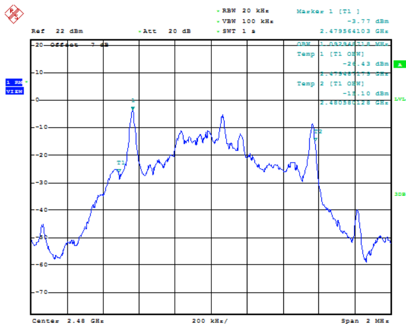
Fig.99 99% Bandwidth: 8DPSK, Ch39
