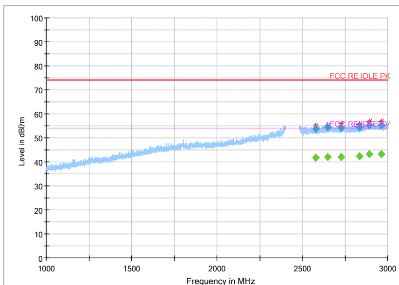
Fig.51 Radiated emission: 8DPSK, Ch78, 1GHz~3GHz
