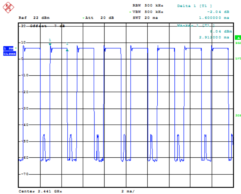
Fig.62 Number of Transmissions Measurement: Ch39, Packet 2-DH1
