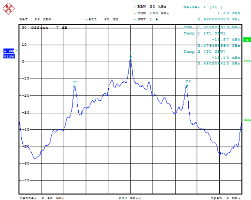
Fig.93 99% Bandwidth: GFSK, Ch39
