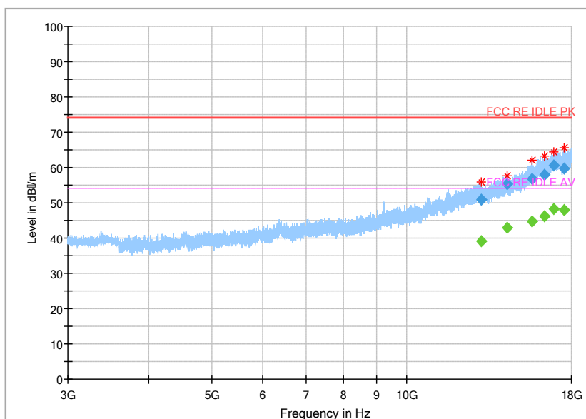
Fig.47 Radiated emission: \pi/4 DQPSK, Ch78, 3GHz~18GHz
