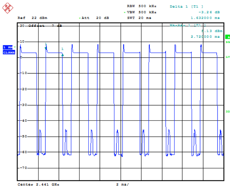
Fig.68 Number of Transmissions Measurement: Ch39, Packet 3-DH1
