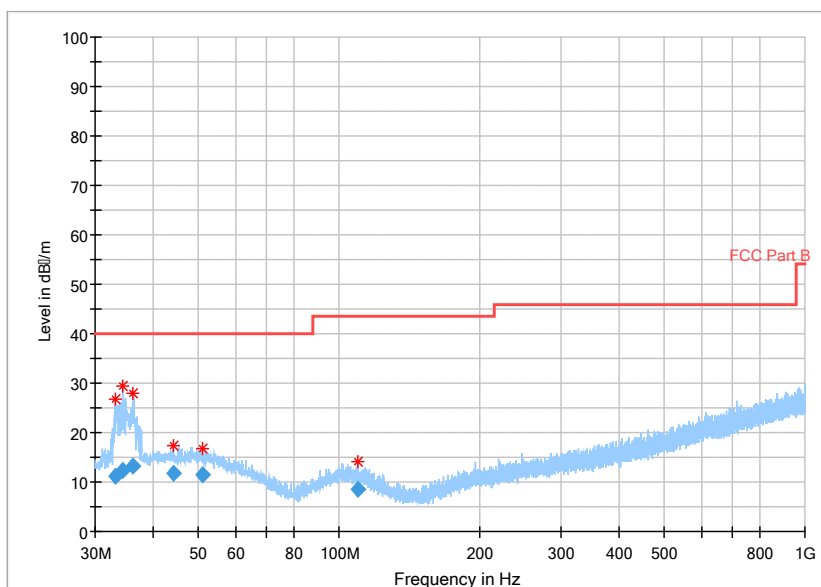
Fig.45 Radiated emission: \pi/4 DQPSK, Ch78, 30MHz~1GHz
