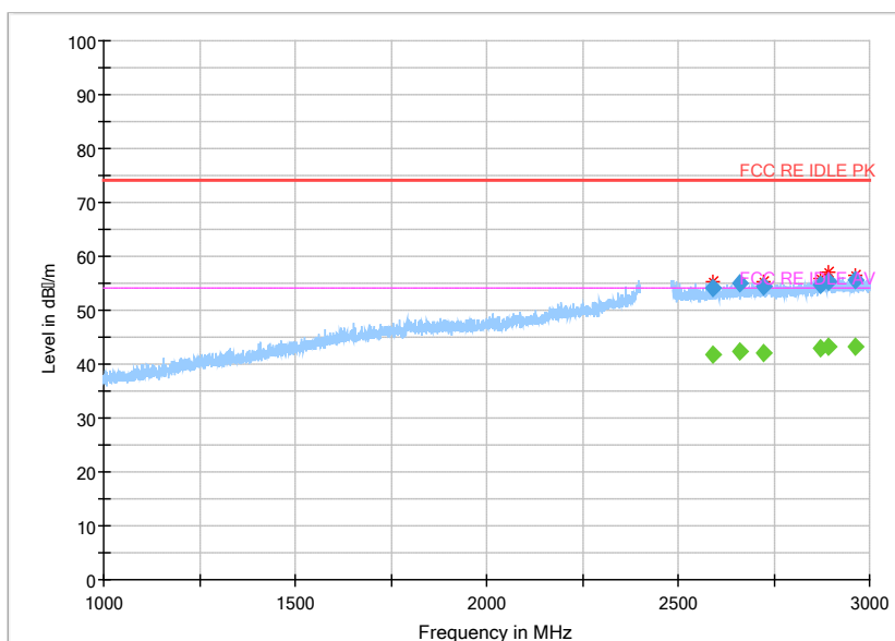
Fig.46 Radiated emission: \pi/4 DQPSK, Ch78, 1GHz~3GHz
