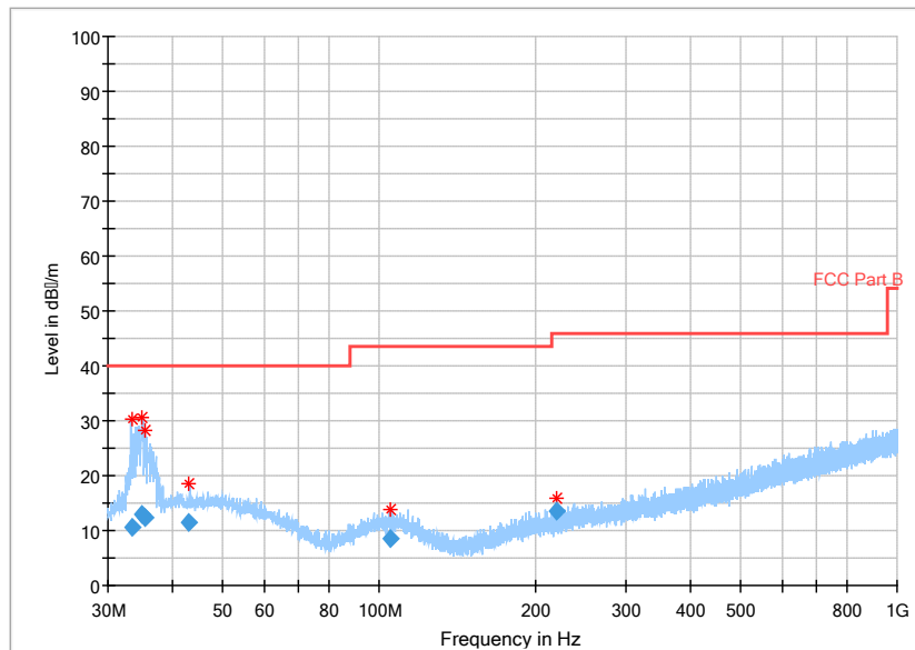
Fig.40 Radiated emission: GFSK, Ch78, 30MHz~1GHz
