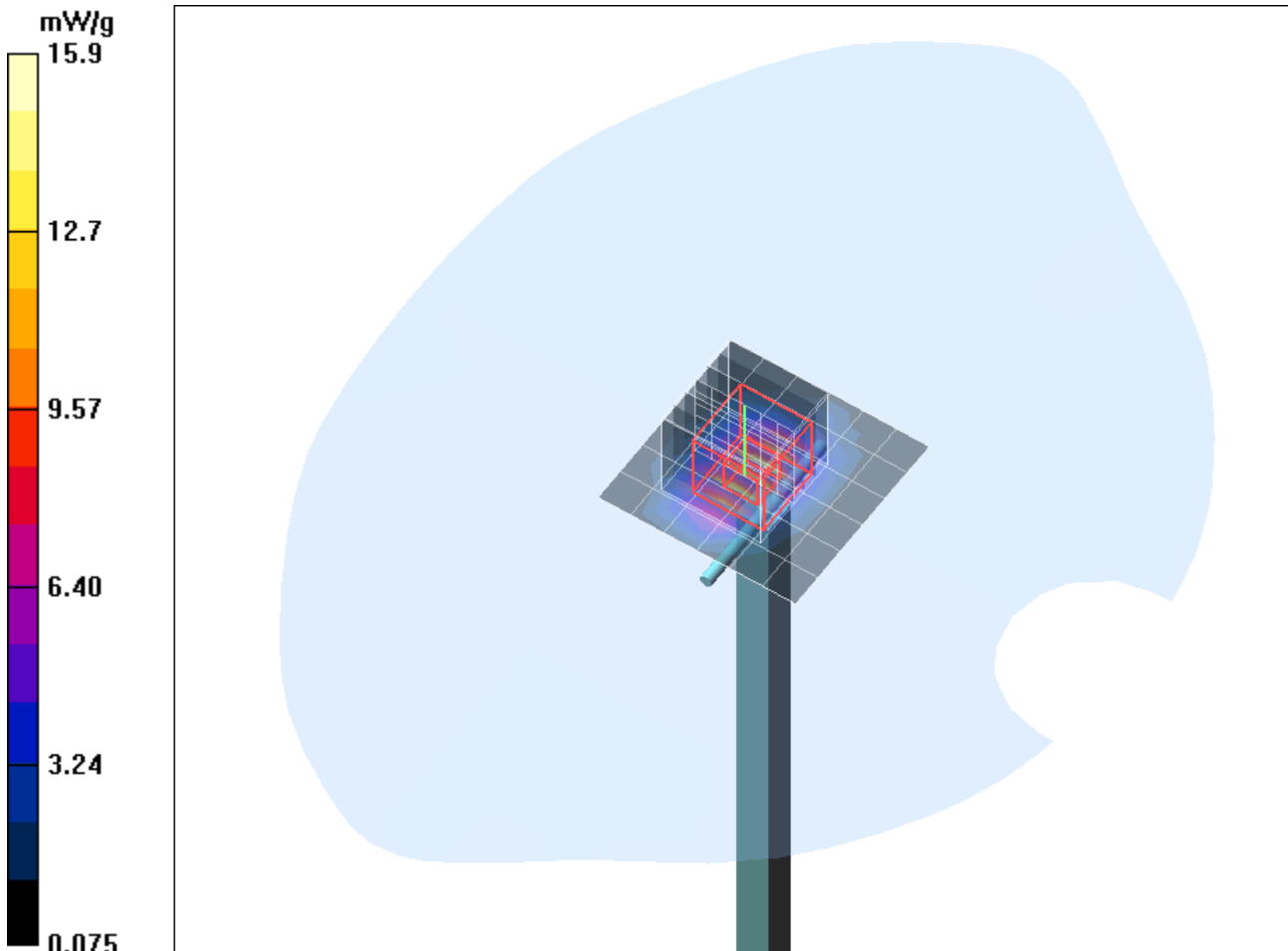
Fig. 8: Validation measurement 2450 MHz Body (September 12, 2013), coarse grid.
