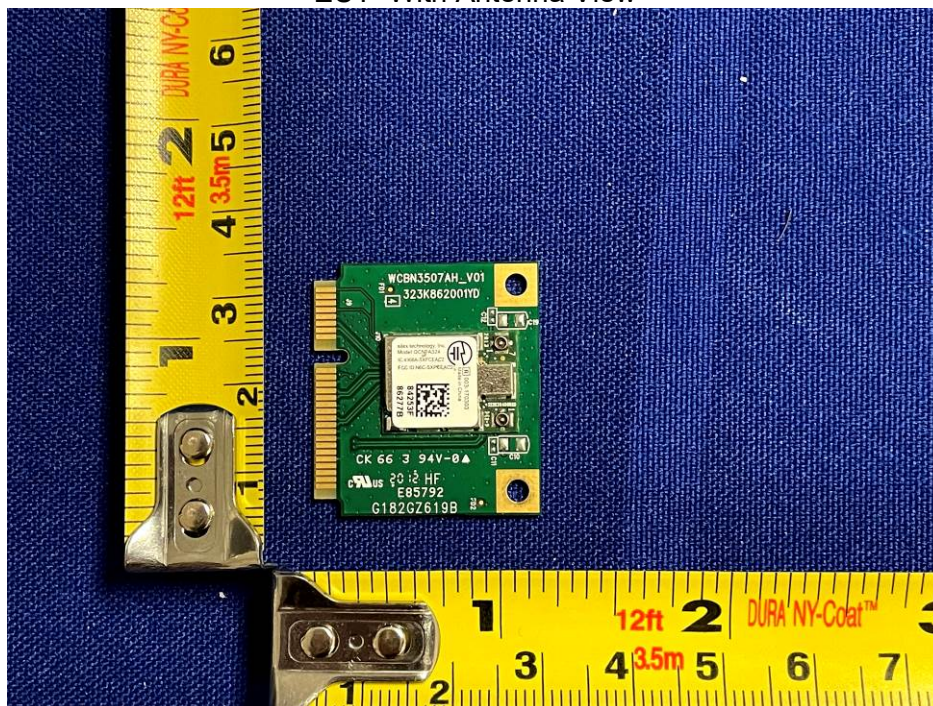
EUT View 1
