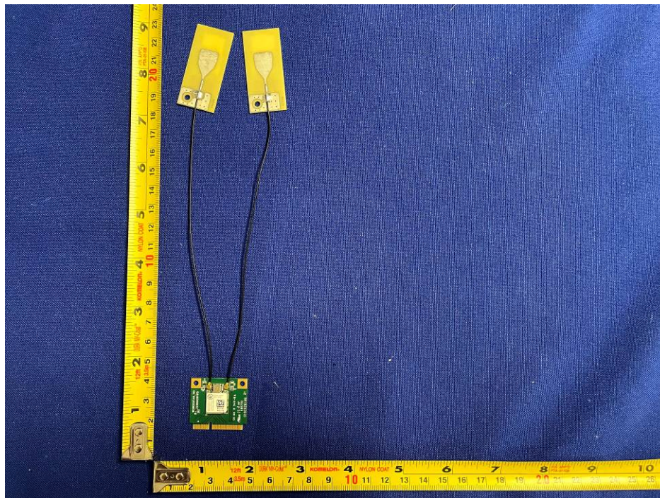
EUT With Antenna View
