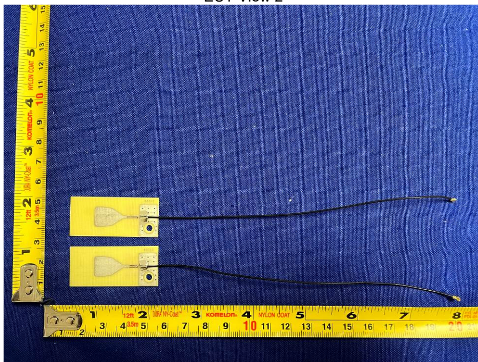
Antenna View 1
