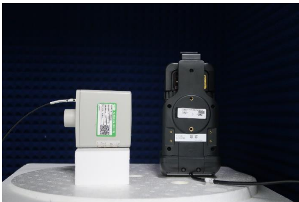
Right Side at 5 cm separation distance
