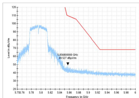
BANDEDGE-11AC(40M)-CH159-PK
