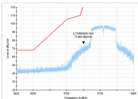
BANDEDGE-11AC(40M)-CH151-PK
