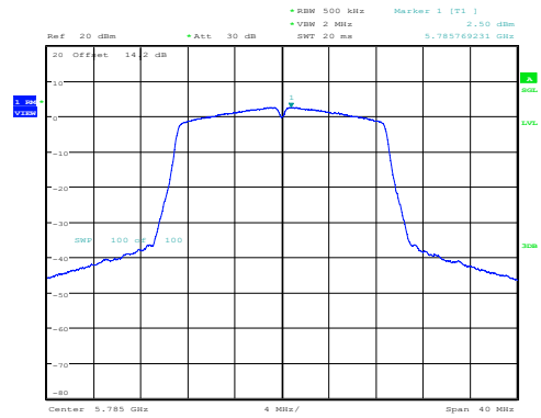
11AC20SISO-Ant1-5785-PASS
