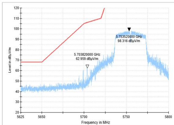
BANDEDGE-11N(40M)-CH151-PK
