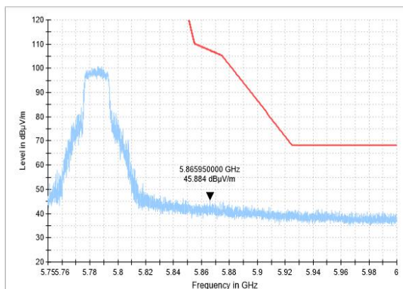
BANDEDGE-11AC-CH157-PK
