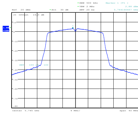
11AC20SISO-Ant1-5745-PASS
