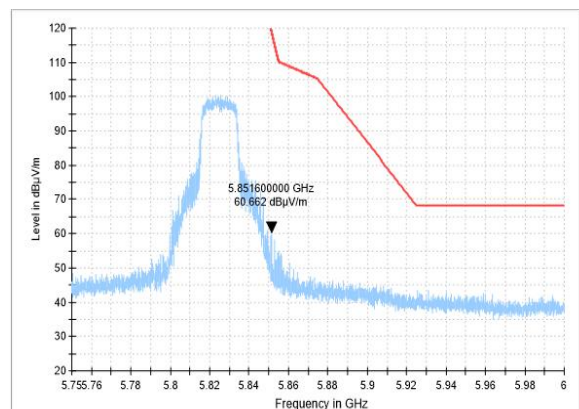
BANDEDGE-11AC-CH165-PK
