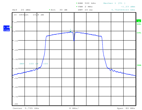
11AC40SISO-Ant1-5755-PASS
