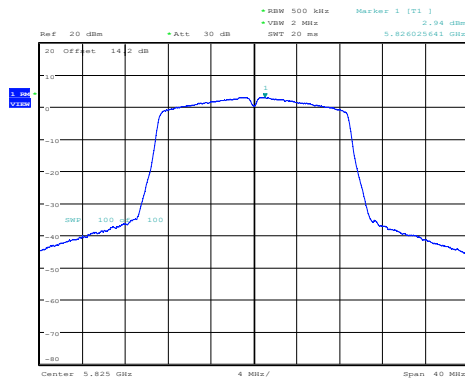
11AC20SISO-Ant1-5825-PASS
