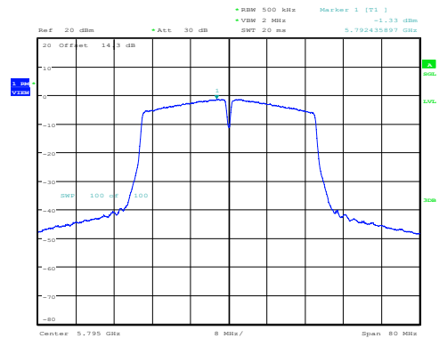
11N40SISO-Ant1-5795-PASS
