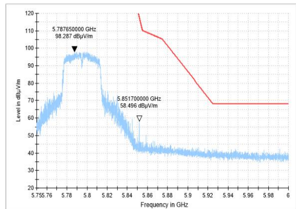
BANDEDGE-11N(40M)-CH159-PK
