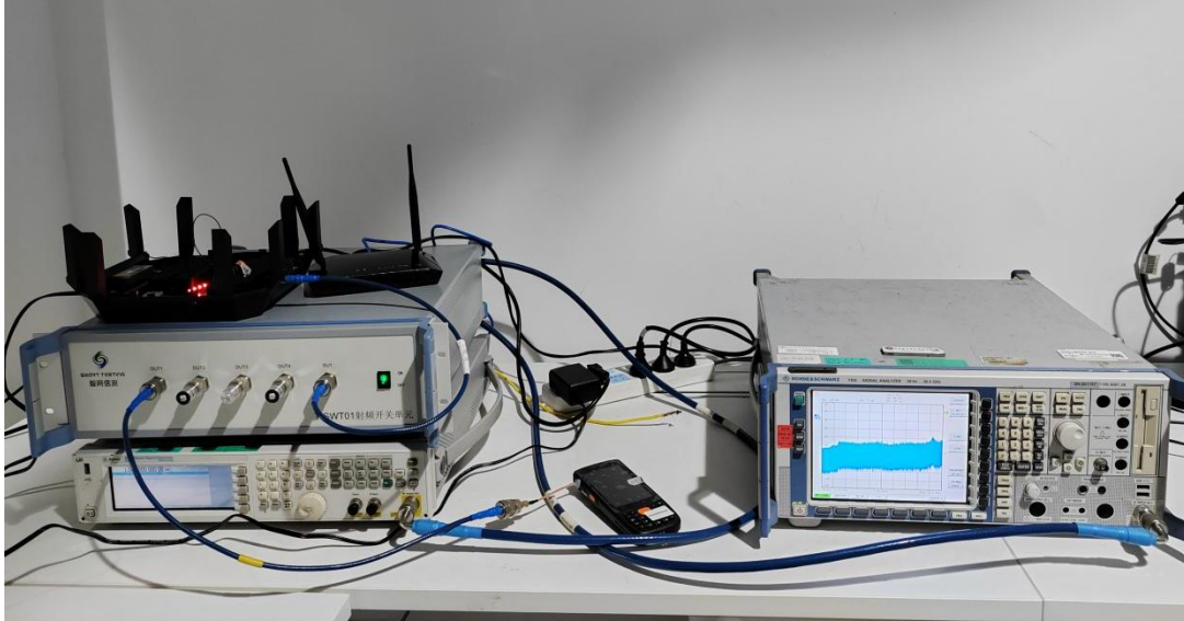
Figure: DFS Set-up Photo
