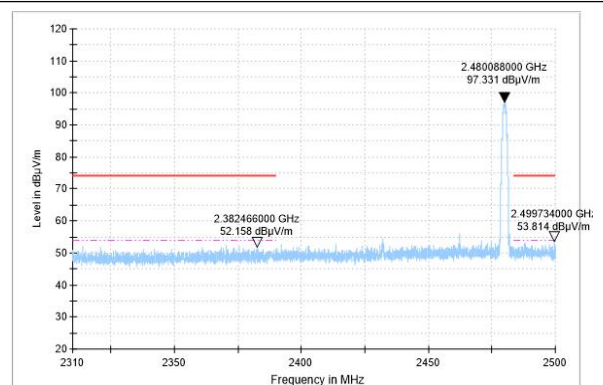
BANDEDGE-2DH5-CH78-PK
