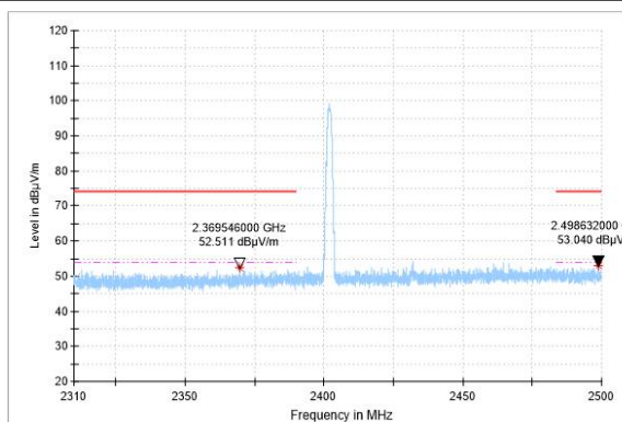
BANDEDGE-3DH5-CH0-PK
