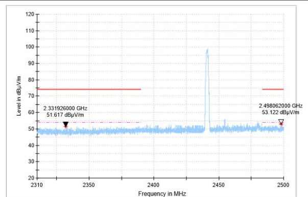
BANDEDGE-3DH5-CH39-PK
