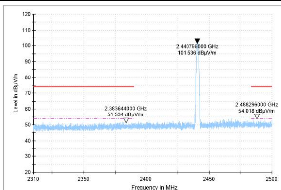
BANDEDGE-2DH5-CH39-PK
