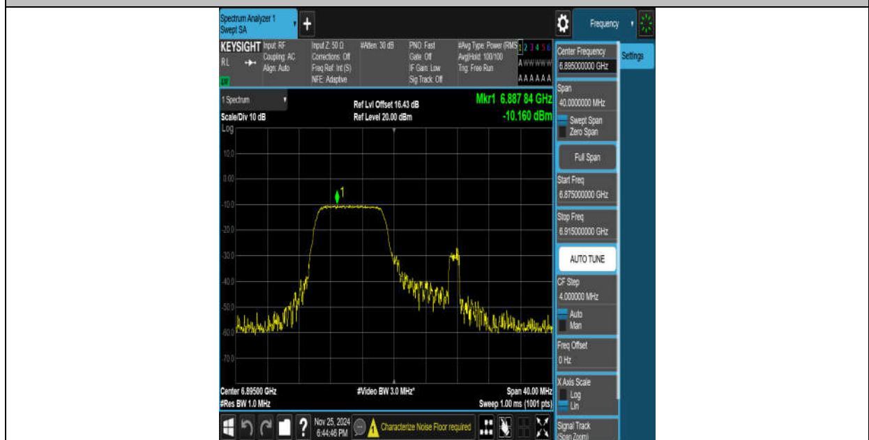
11AX20MIMO-Ant9-6895-106Tone-RU53-PASS
