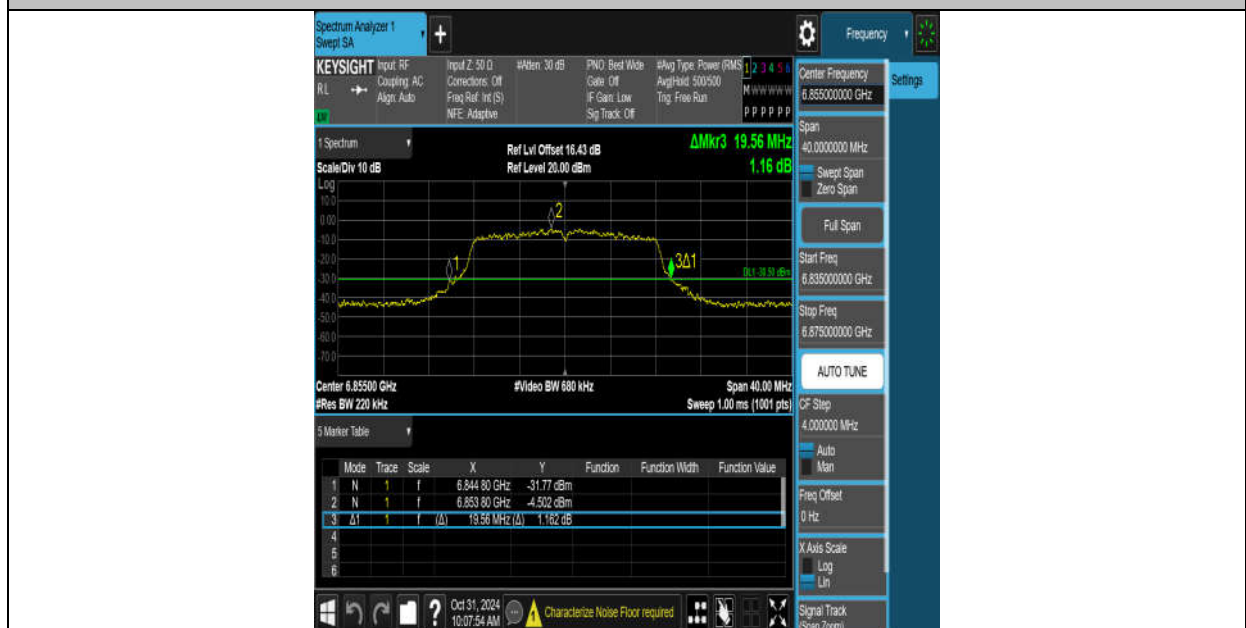
11A-Ant9-6855
