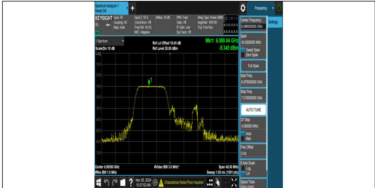
11AX20MIMO-Ant8-6995-106Tone-RU53-PASS
