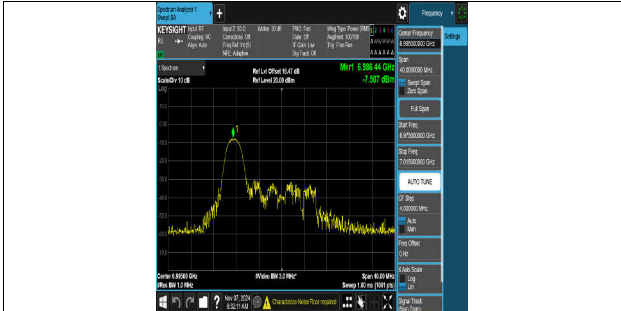
11AX20MIMO-Ant9-6995-26Tone-RU0-PASS
