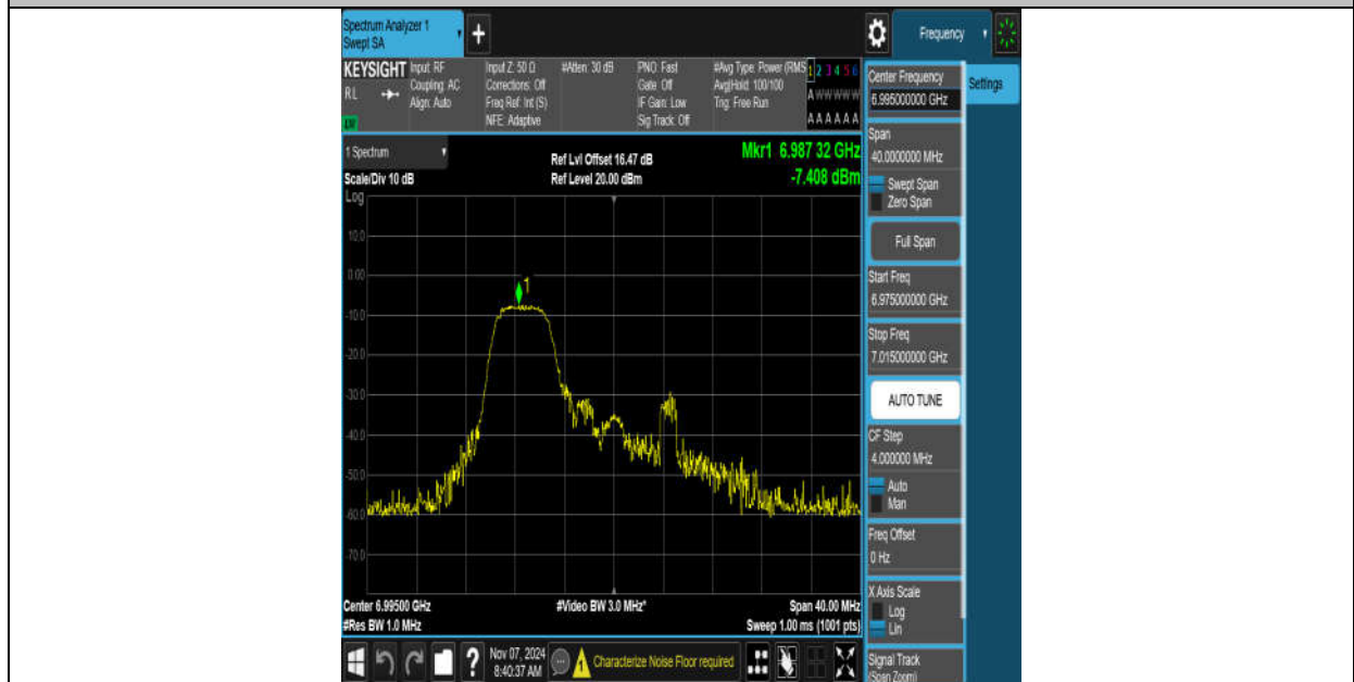
11AX20MIMO-Ant9-6995-52Tone-RU37-PASS
