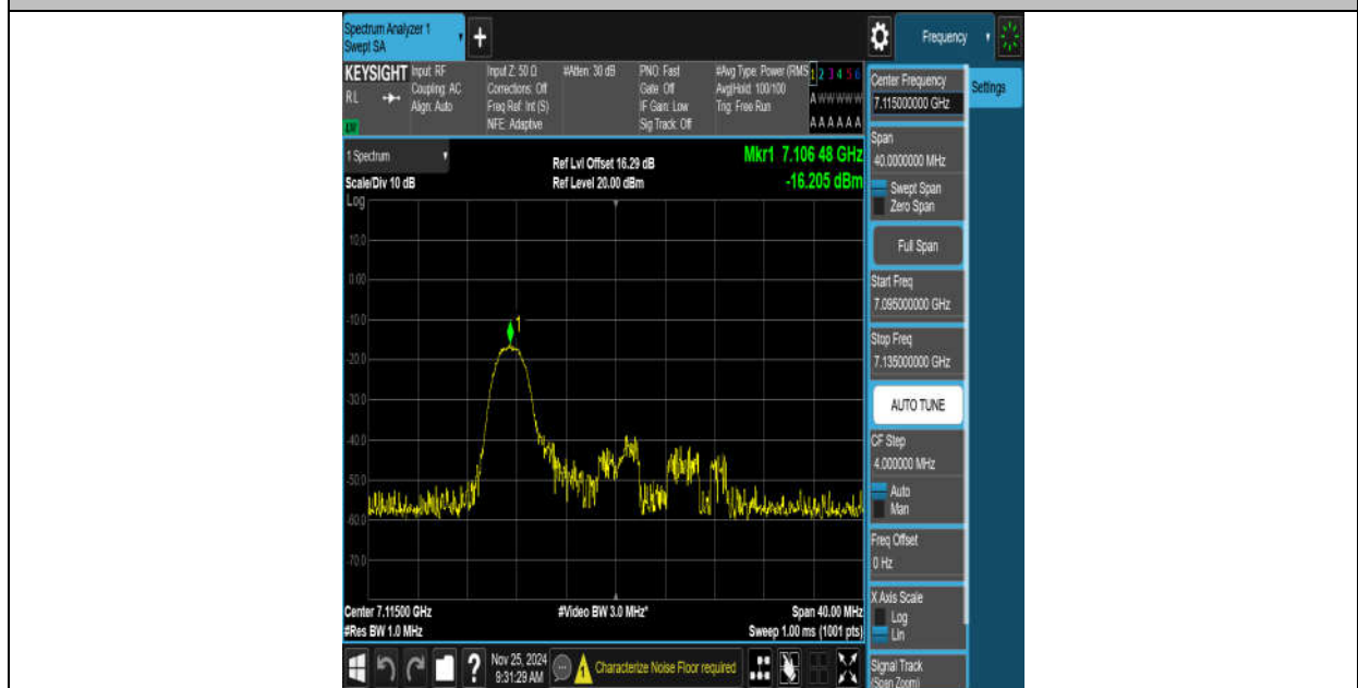
11AX20MIMO-Ant9-7115-26Tone-RU0-PASS
