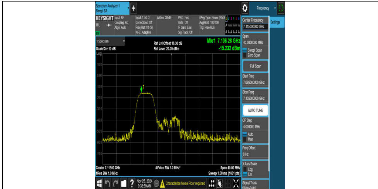
11AX20MIMO-Ant8-7115-52Tone-RU37-PASS
