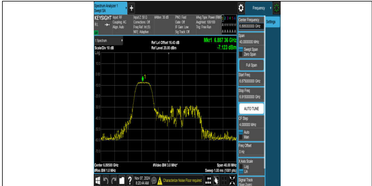
11AX20MIMO-Ant8-6895-52Tone-RU37-PASS
