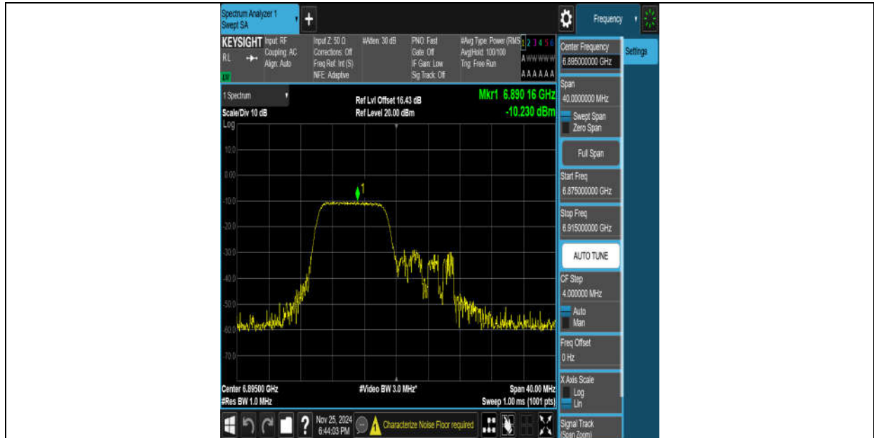
11AX20MIMO-Ant8-6895-106Tone-RU53-PASS
