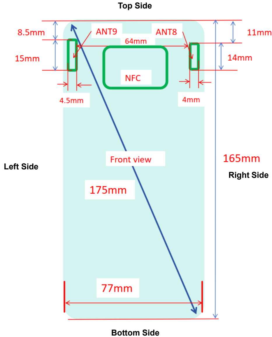
Picture 11.1 Antenna Locations (Front View)
