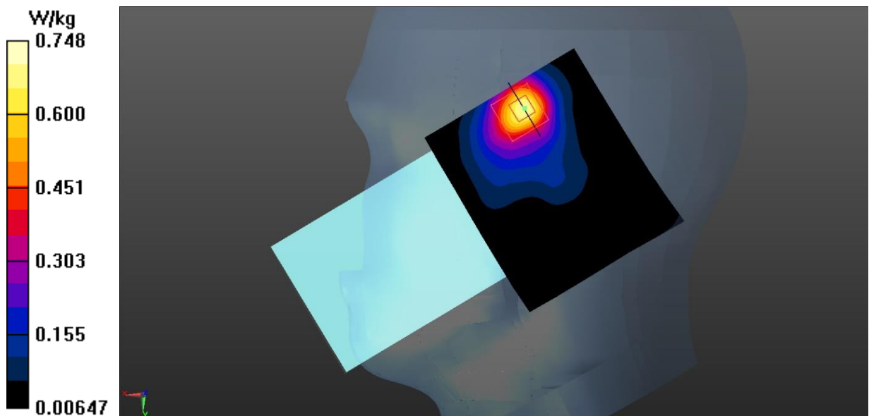
Fig.4 WLAN 2.4GHz Head
