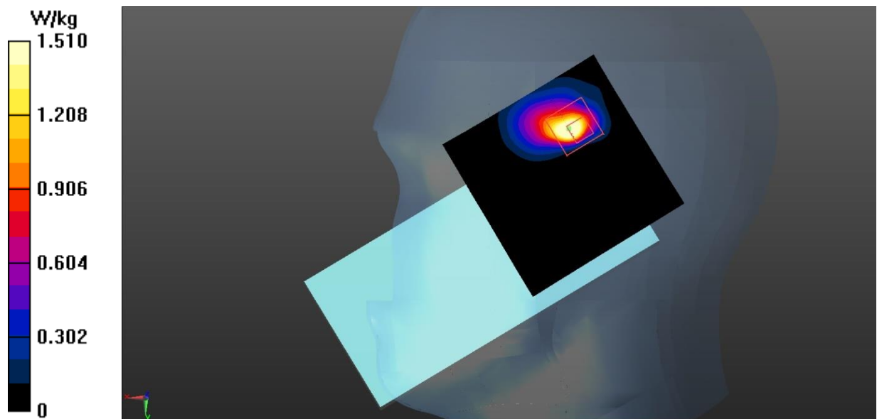
Fig.7 WLAN 5GHz Head
