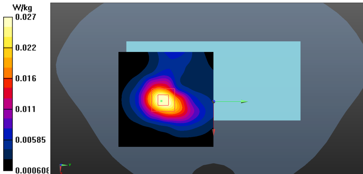
Fig.2 Bluetooth Body
