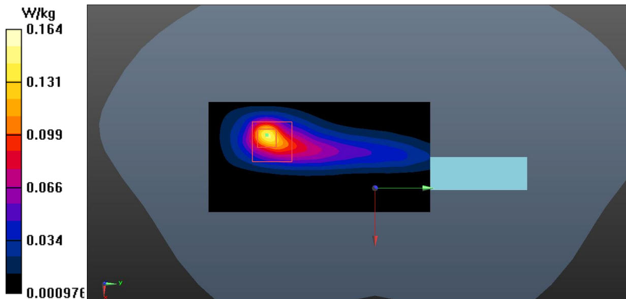
Fig.3 Bluetooth Extremity
