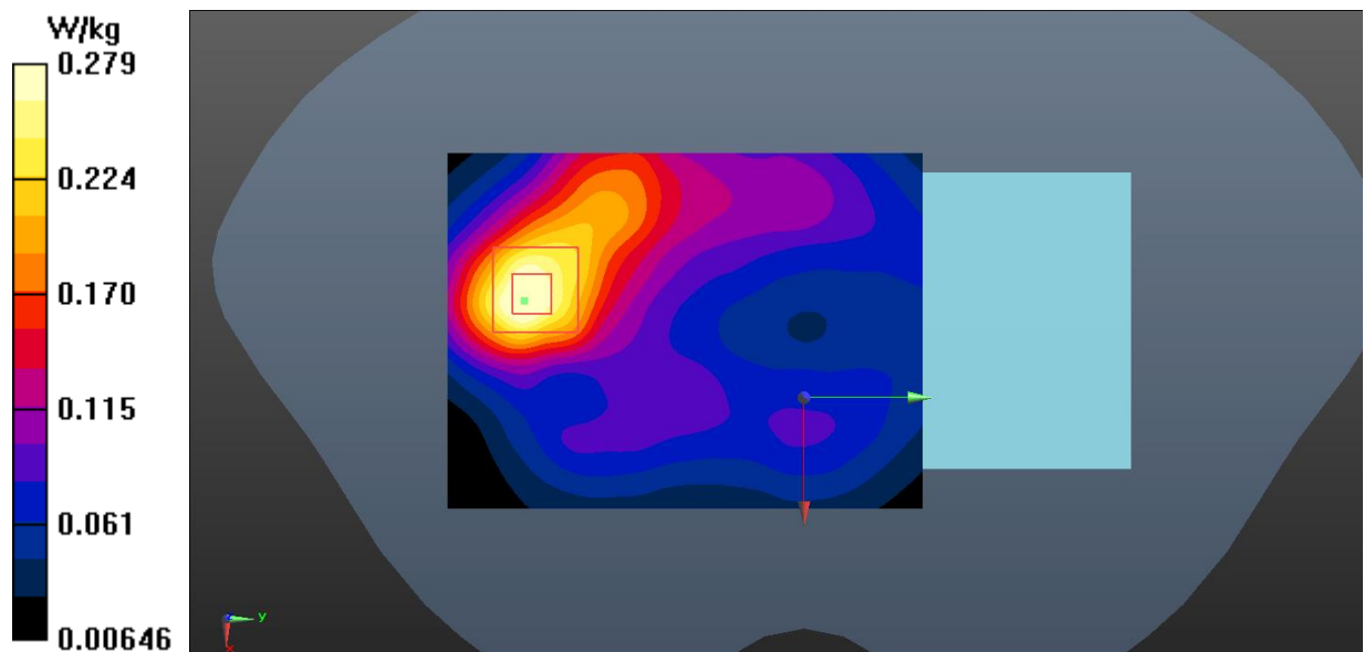
Fig.5 WLAN 2.4GHz Body
