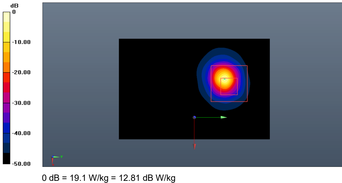
Fig.B.3. Validation 5250MHz 100mW
