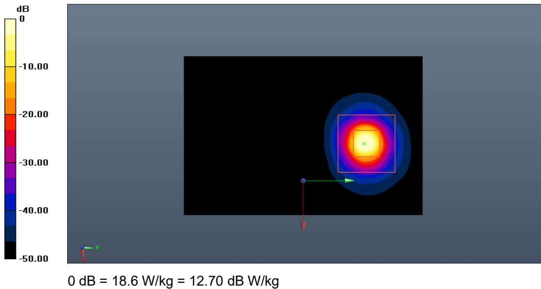
Fig.B.4. Validation 5600MHz 100mW
