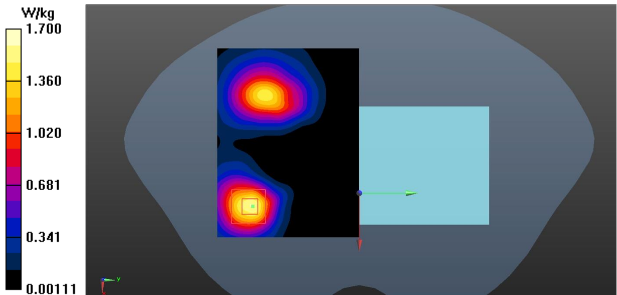
Fig.8 WLAN 5GHz Body
