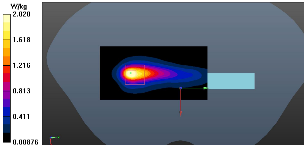
Fig.6 WLAN 2.4GHz Extremity
