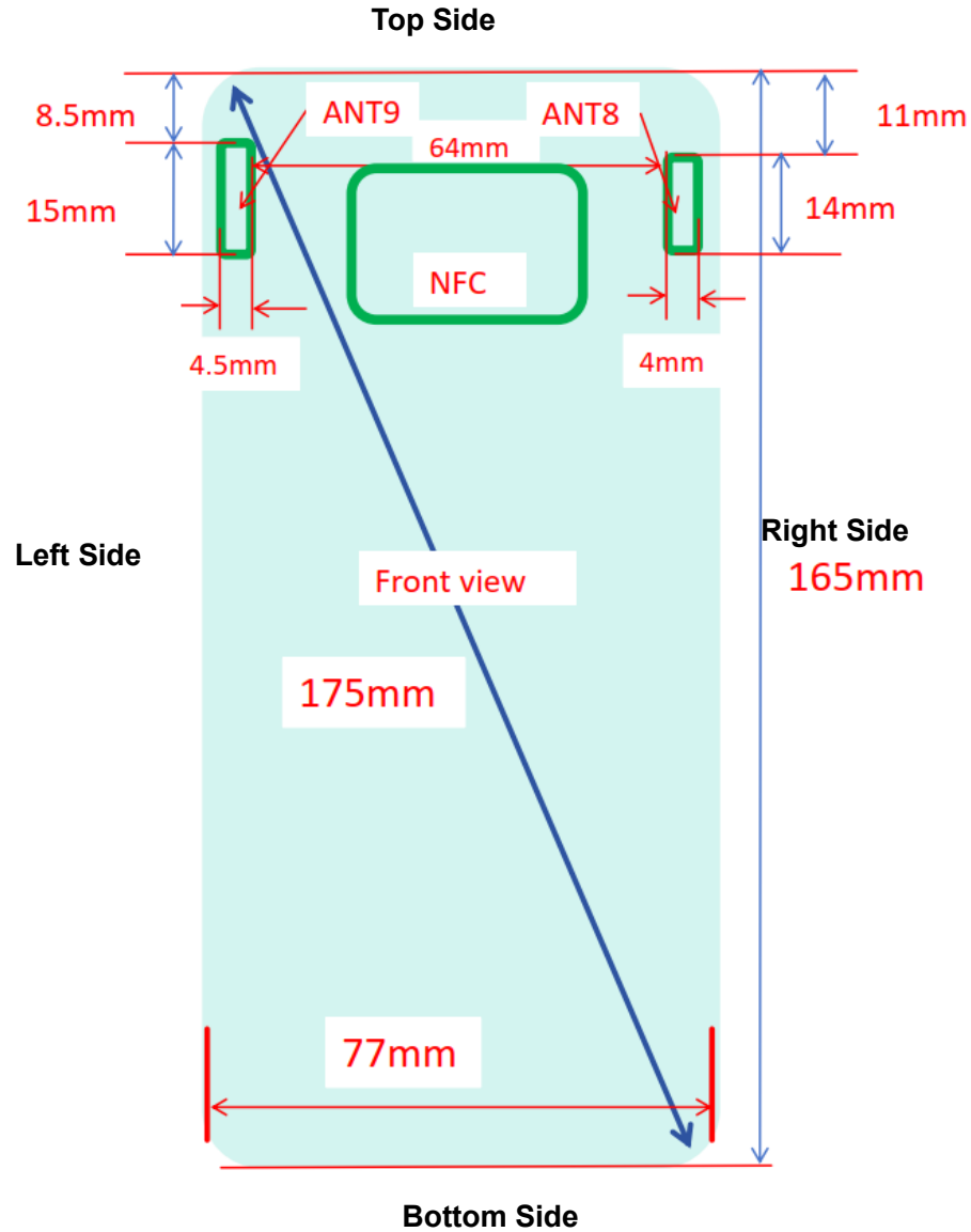
Picture 11.1 Antenna Locations (Front View)
