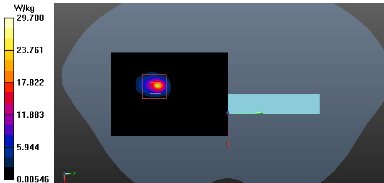
Fig.9 WLAN 5GHz Extremity
