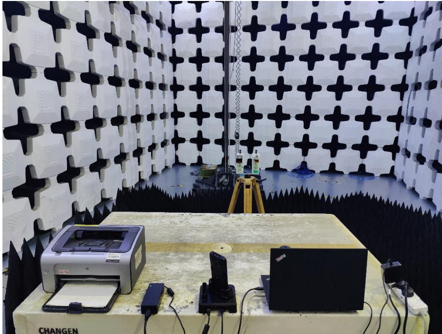
7. Radiated Emissions (Part 15B, Charging via POGO PIN/ Data Transfer, 18GHz-26.5GHz)
