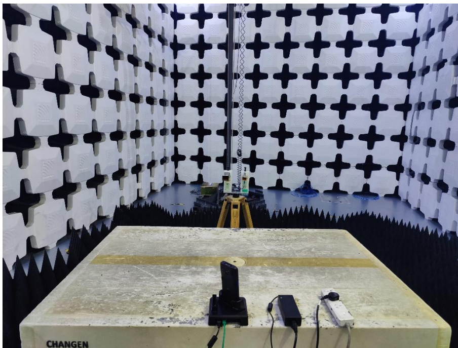
24. Radiated Emissions (Part 15B Charging via POGO PIN/Ethernet Connection,26.5GHz-40GHz)
