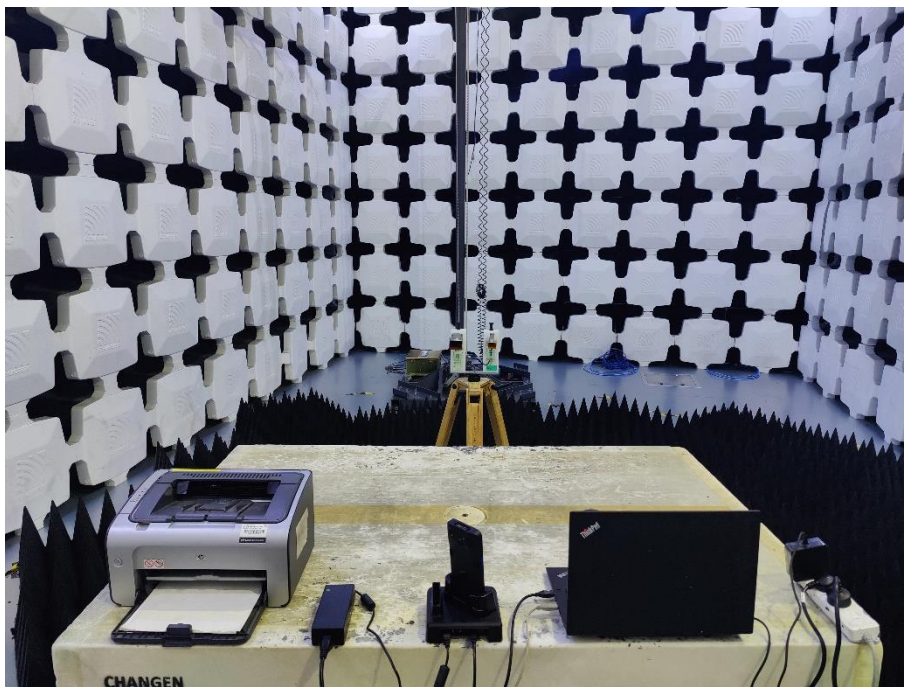
8. Radiated Emissions (Part 15B, Charging via POGO PIN/ Data Transfer, 26.5GHz-40GHz)
