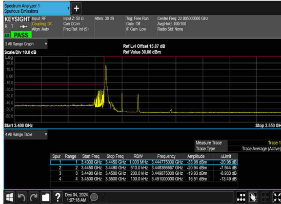
N77(20M)_DFT-s- OFDM_BPSK_Edge_1RB_Left_Low_CH
