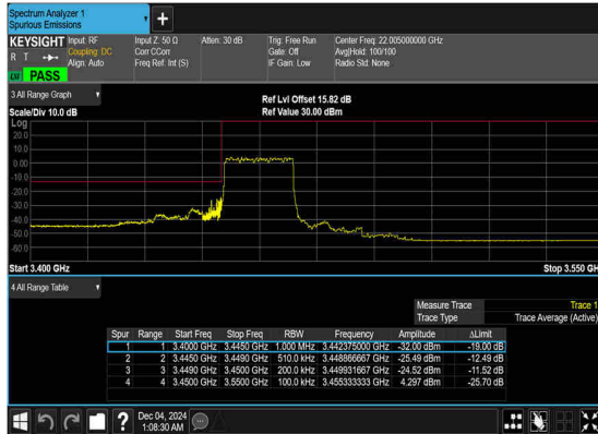
N77(20M)_DFT-s- OFDM_BPSK_Outer_Full_Low_CH
