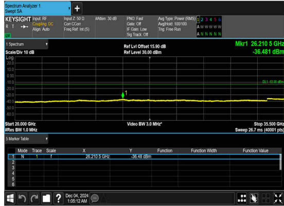
N77(100M)_DFT-s-OFDM_BPSK_Edge_1RB_Left_Mid_CH
