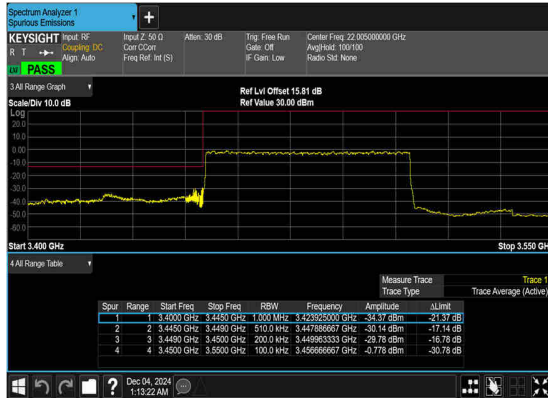
N77(60M)_DFT-s- OFDM_BPSK_Outer_Full_Low_CH
