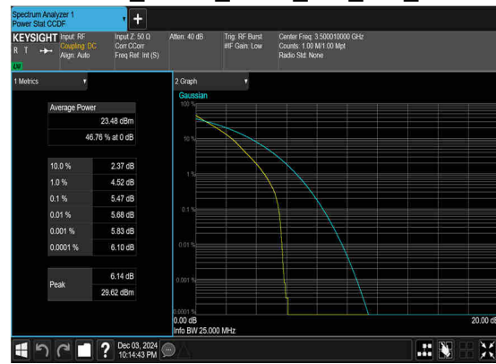
N77(20M)_DFT-s-OFDM_QPSK_Outer_Full_Mid_CH
