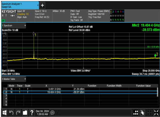
N77(60M)_DFT-s-OFDM_BPSK_Edge_1RB_Left_High_CH
