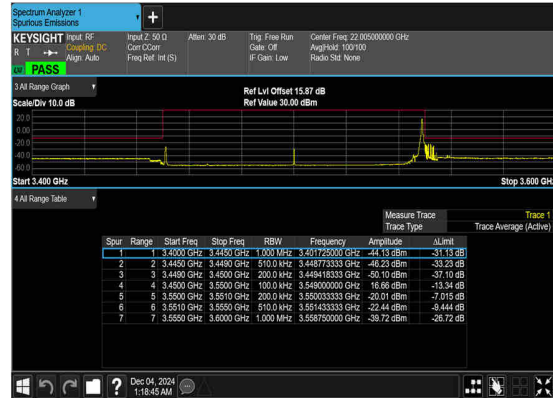
N77(100M)_DFT-s- OFDM_QPSK_Edge_1RB_Right_Mid_CH
