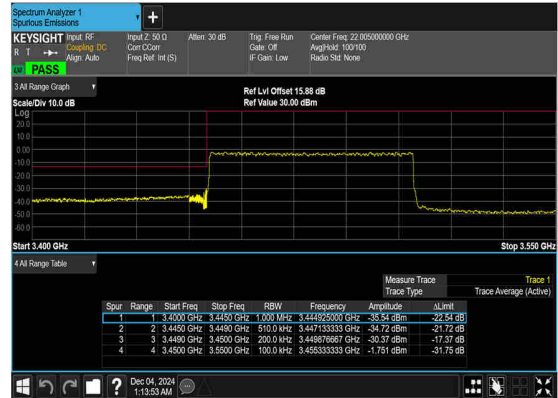
N77(60M)_DFT-s- OFDM_QPSK_Outer_Full_Low_CH
