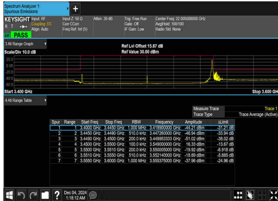
N77(100M)_DFT-s- OFDM_BPSK_Edge_1RB_Right_Mid_CH
