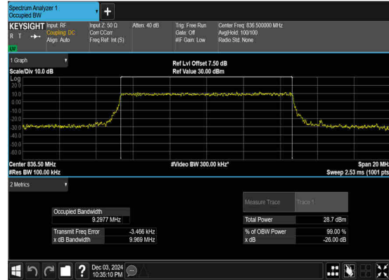
N5(10M)_CP-OFDM_16 QAM_Outer_Full_Mid_CH
