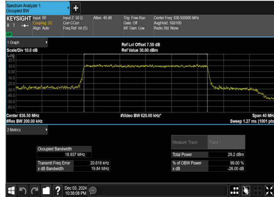
N5(20M)_CP-OFDM_16 QAM_Outer_Full_Mid_CH
