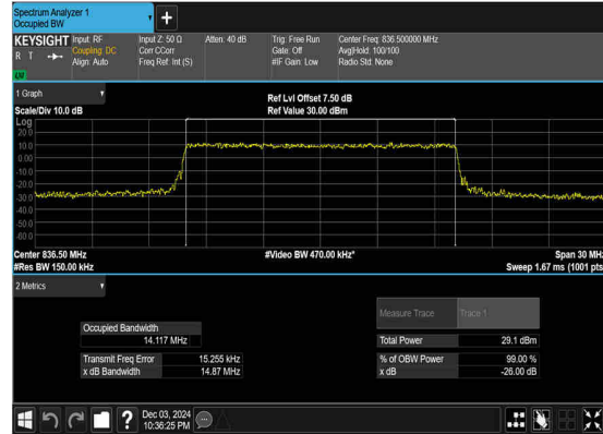
N5(15M)_CP-OFDM_16 QAM_Outer_Full_Mid_CH
