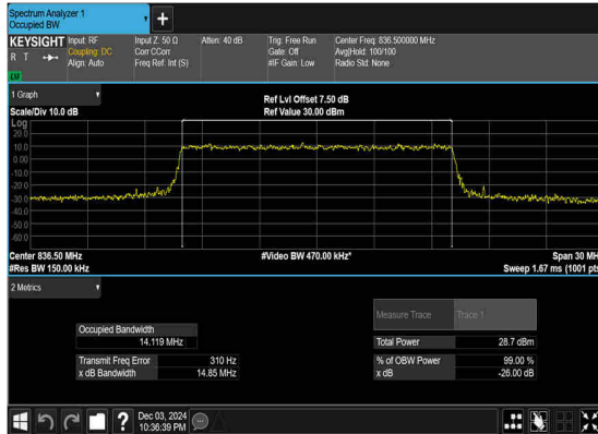
N5(15M)_CP-OFDM_64 QAM_Outer_Full_Mid_CH
