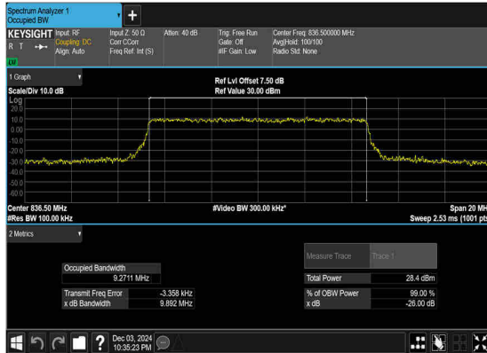
N5(10M)_CP-OFDM_64 QAM_Outer_Full_Mid_CH
