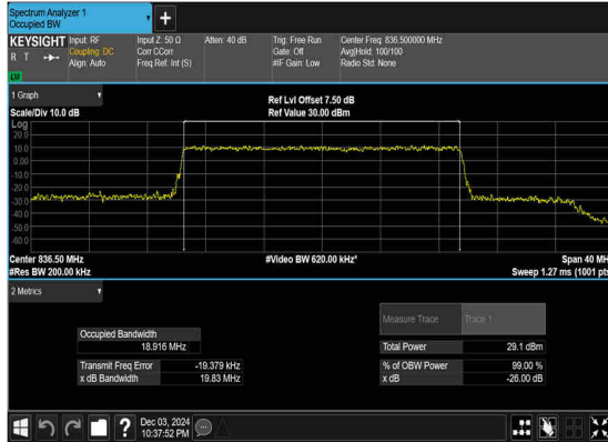
N5(20M)_CP- OFDM_QPSK_Outer_Full_Mid_CH
