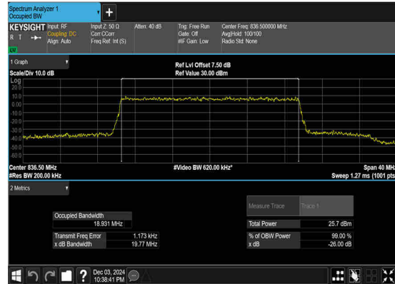
N5(20M)_CP-OFDM_256 QAM_Outer_Full_Mid_CH
