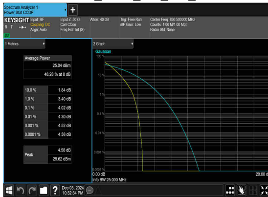
N5(20M)_DFT-s-OFDM_PI_2-BPSK_Outer_Full_Mid_CH
