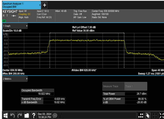
N5(20M)_CP-OFDM_64 QAM_Outer_Full_Mid_CH
