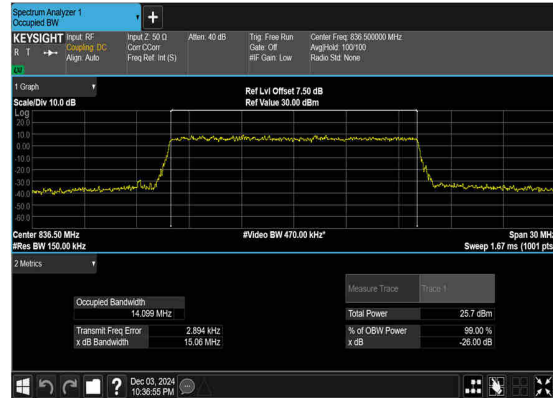
N5(15M)_CP-OFDM_256 QAM_Outer_Full_Mid_CH
