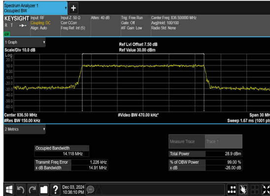
N5(15M)_CP- OFDM_QPSK_Outer_Full_Mid_CH
