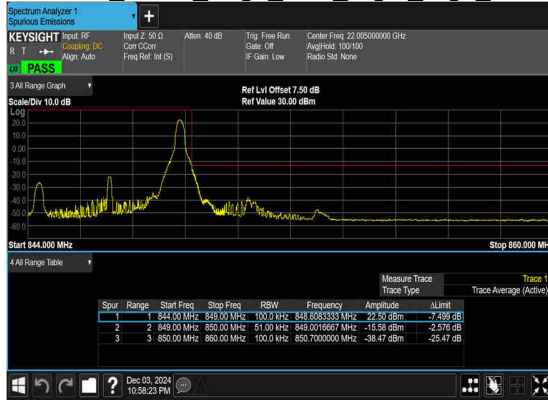
N5(5M)_DFT-s- OFDM BPSK Edge 1RB Right High CH
