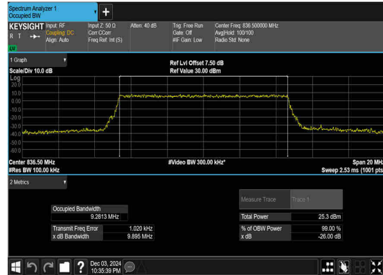
N5(10M)_CP-OFDM_256 QAM_Outer_Full_Mid_CH
