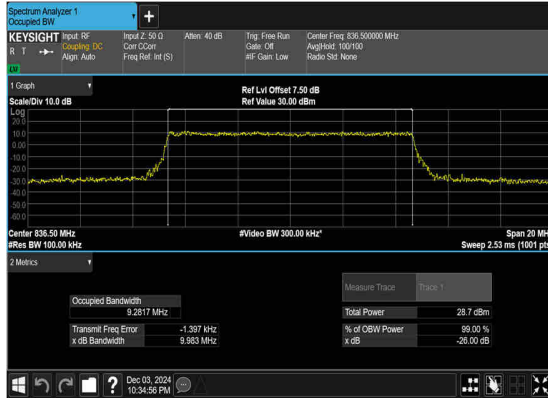
N5(10M)_CP- OFDM_QPSK_Outer_Full_Mid_CH
