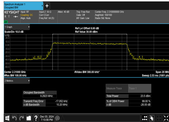
N30(10M)_CP-OFDM_256 QAM_Outer_Full_Low_CH
