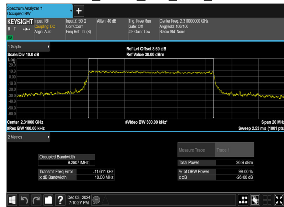
N30(10M)_CP-OFDM_16 QAM_Outer_Full_Low_CH
