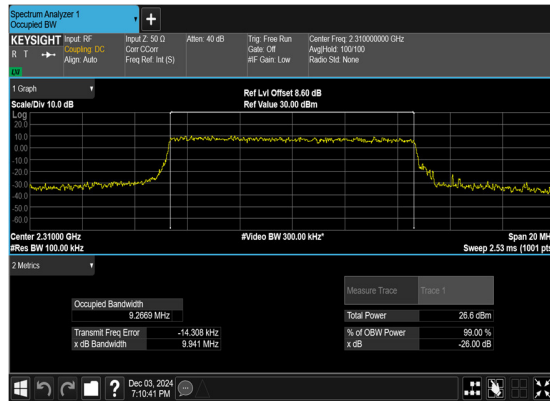
N30(10M)_CP-OFDM_64 QAM_Outer_Full_Low_CH
