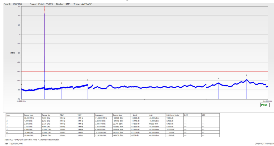
N30(10M)_DFT-s-OFDM_BPSK_Edge_1RB_Left_Low_CH
