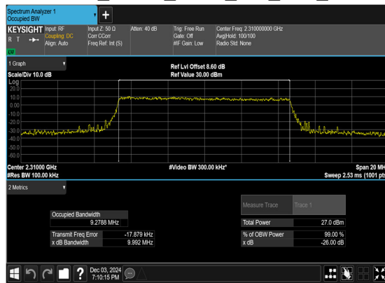
N30(10M)_CP-OFDM_QPSK_Outer_Full_Low_CH
