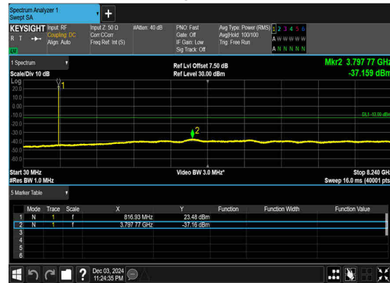
N26(5M)_DFT-s- OFDM_QPSK_Edge_1RB_Left_Mid_CH
