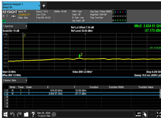
N26(5M)_DFT-s- OFDM_BPSK_Edge_1RB_Left_Mid_CH
