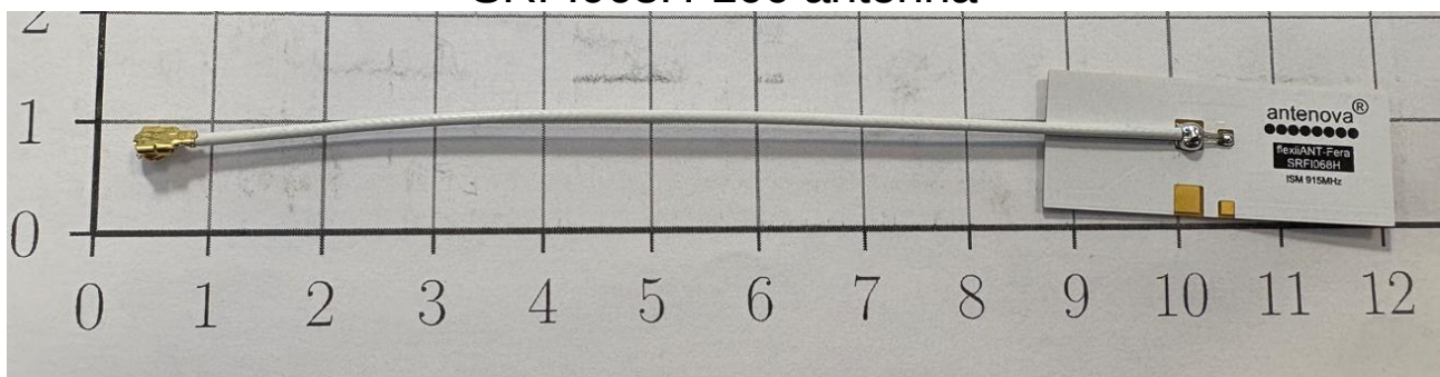
SRFI068H-100 antenna
