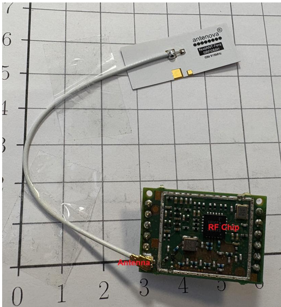
SRFI068H-100 antenna
