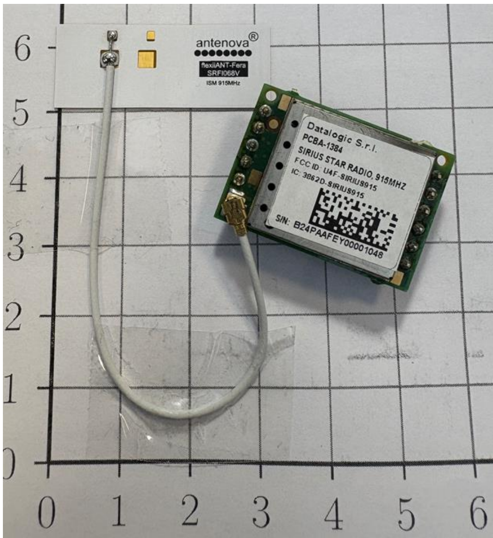
Bottom side with SRFI068V-100 antenna
