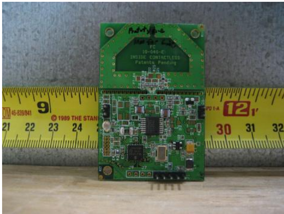
RF MAIN BOARD – COMPONENT SIDE
