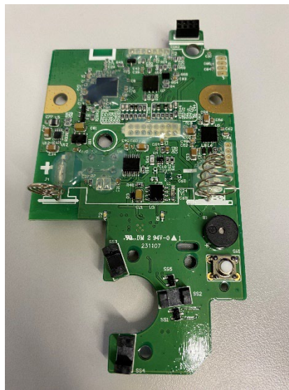
PCB Front
