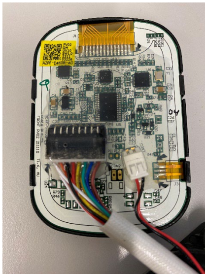
PCB Back
