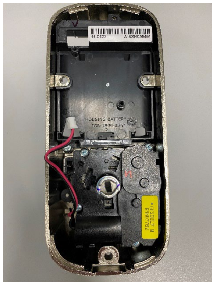
Sub-Assembly with PCB removed
