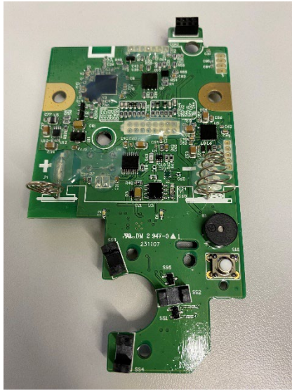
PCB Front
