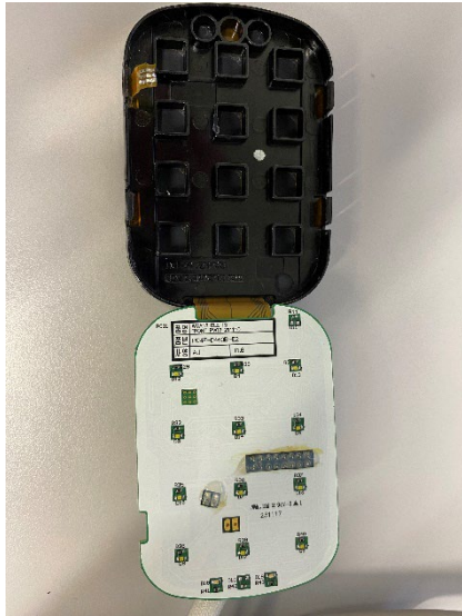
Touchscreen Back, PCB Front
