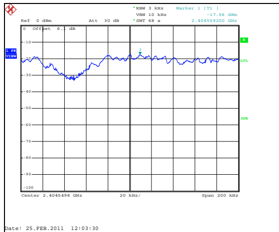
Figure 7.6.2-1: Power Spectral Density Plot – 2405MHz
