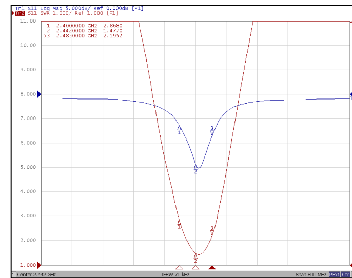
Return Loss & VSWR – WGA13
