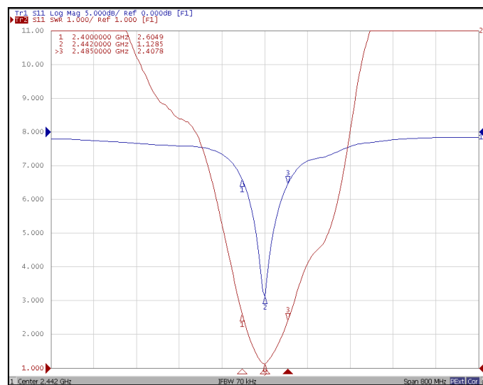
Return Loss & VSWR – WGA10
