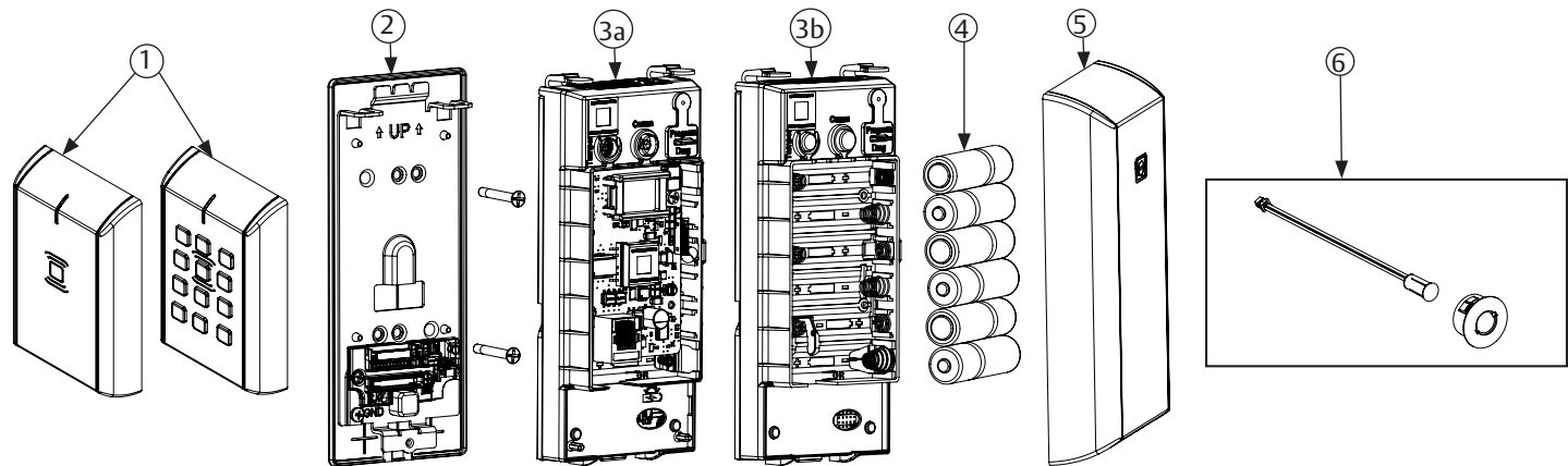
IN120/220 Assembly
