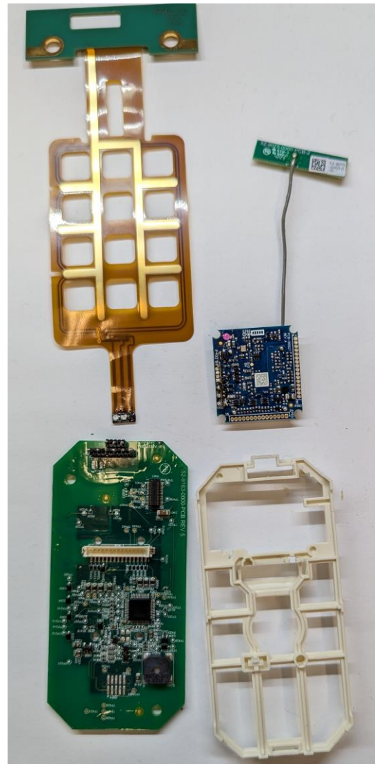
Figure 1 IN120/IN220 PCB Assembly BOTTOM
