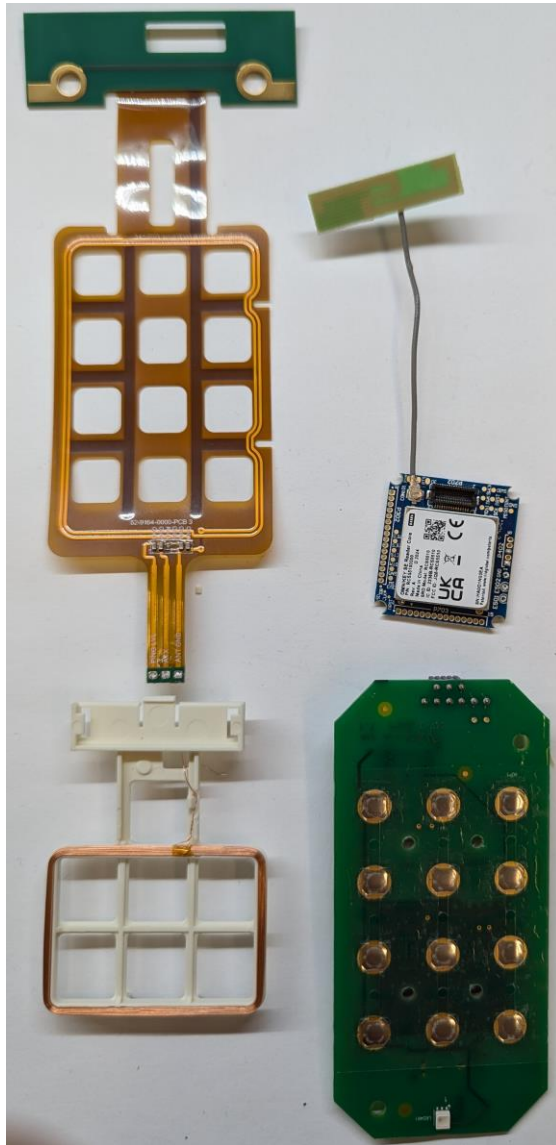
Figure 2 IN120/IN220 PCB Assembly TOP
