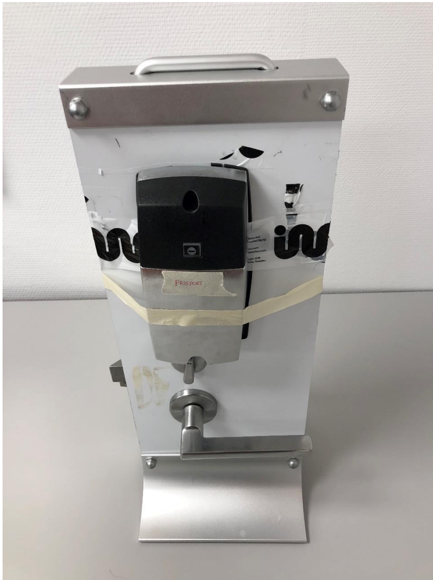
Photo of EUT mounted on door stand with cover 1, frontside.
