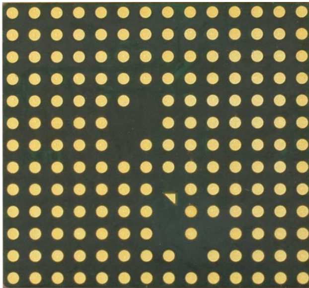
RS9116 Radio Module BOTTOM
