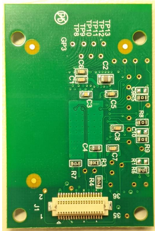
Radio Module Assembly BOTTOM 52-9134
