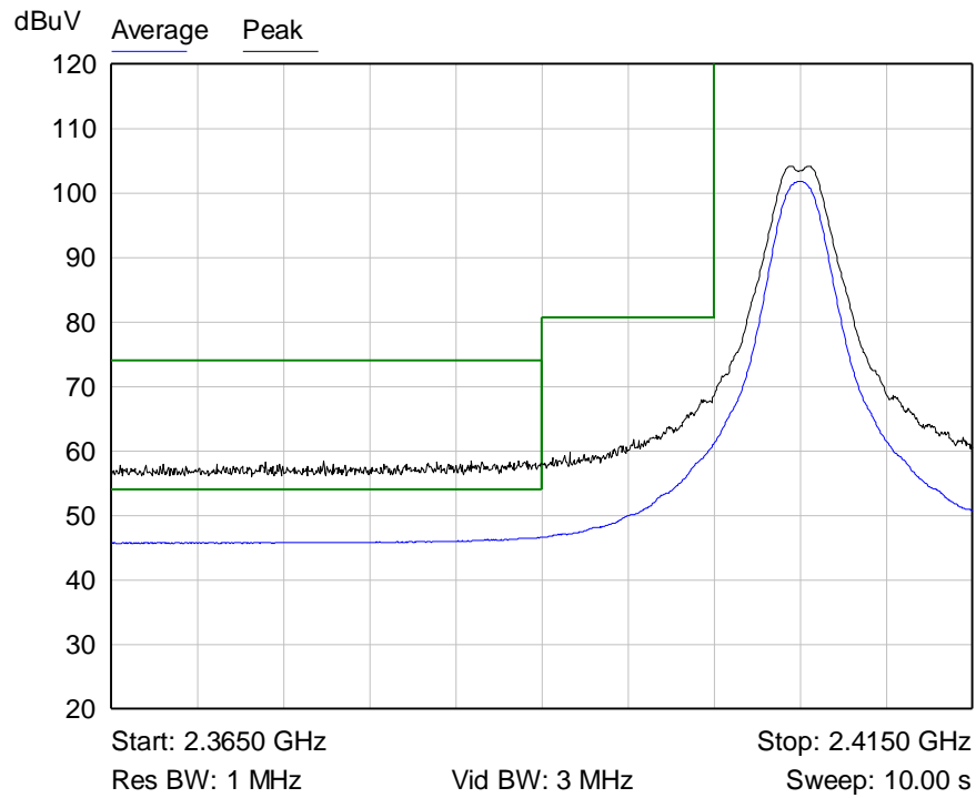
Graph 7: Radiated Lower Band Edge Plot
