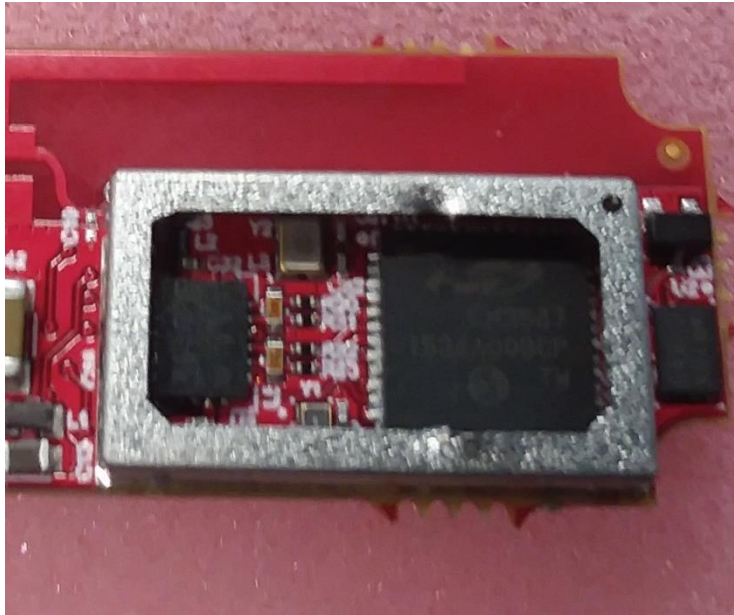
Photograph 13: Circuitry Under the RF Shield
