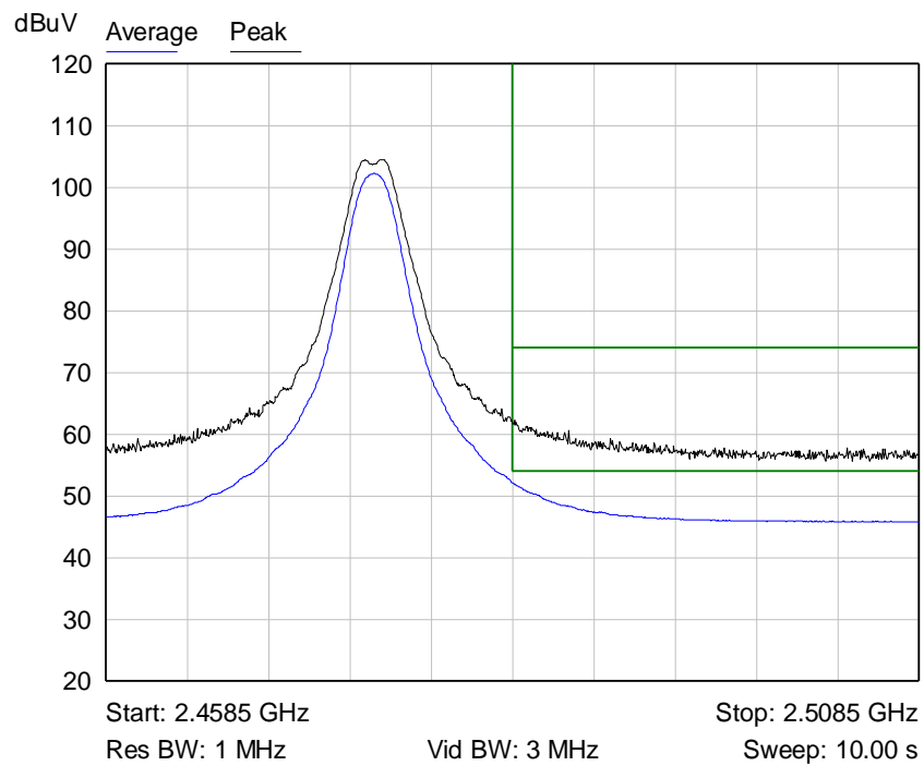
Graph 8: Radiated Upper Band Edge Plot
