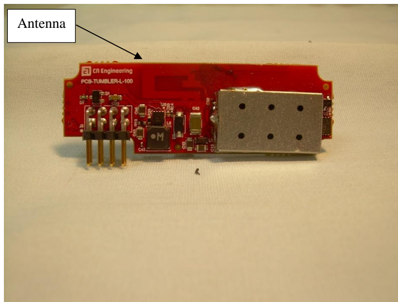
Photograph 12: Front Side of the PCB
