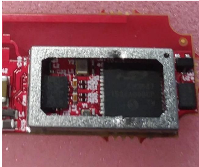
Photograph 3 – View of the Circuitry under the RF Shield
