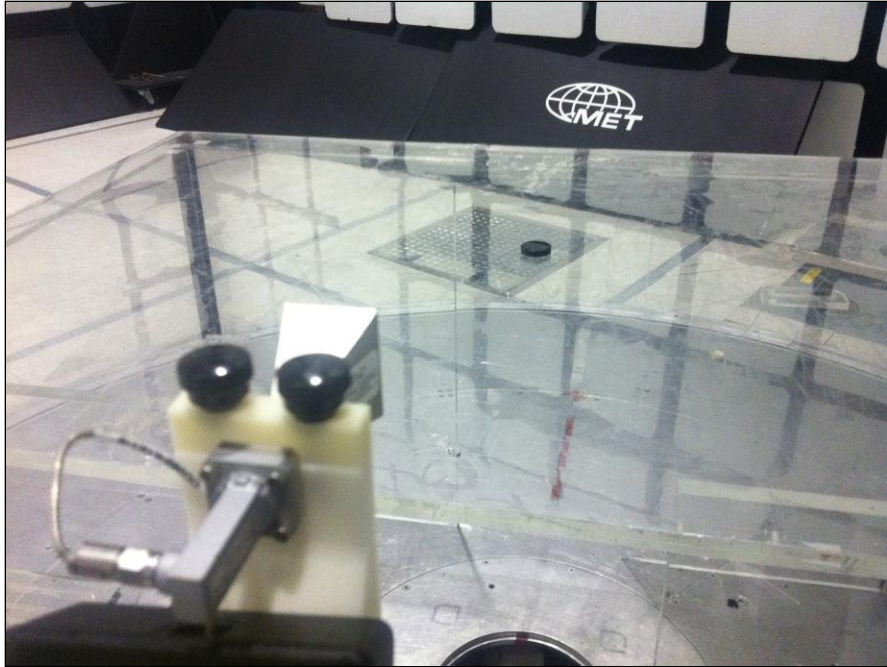
Photograph 5. Radiated Spurious Emissions, Test Setup, 18 GHz – 26 GHz
