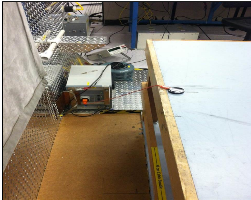
Photograph 2. Conducted Emissions, 15.207(a), Test Setup, Rear View
