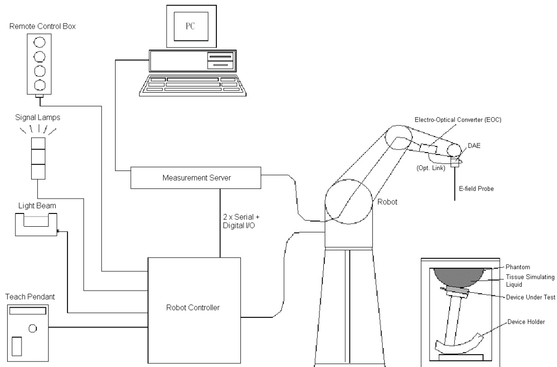
Fig 5.1 SPEAG DASY5 System Configurations
