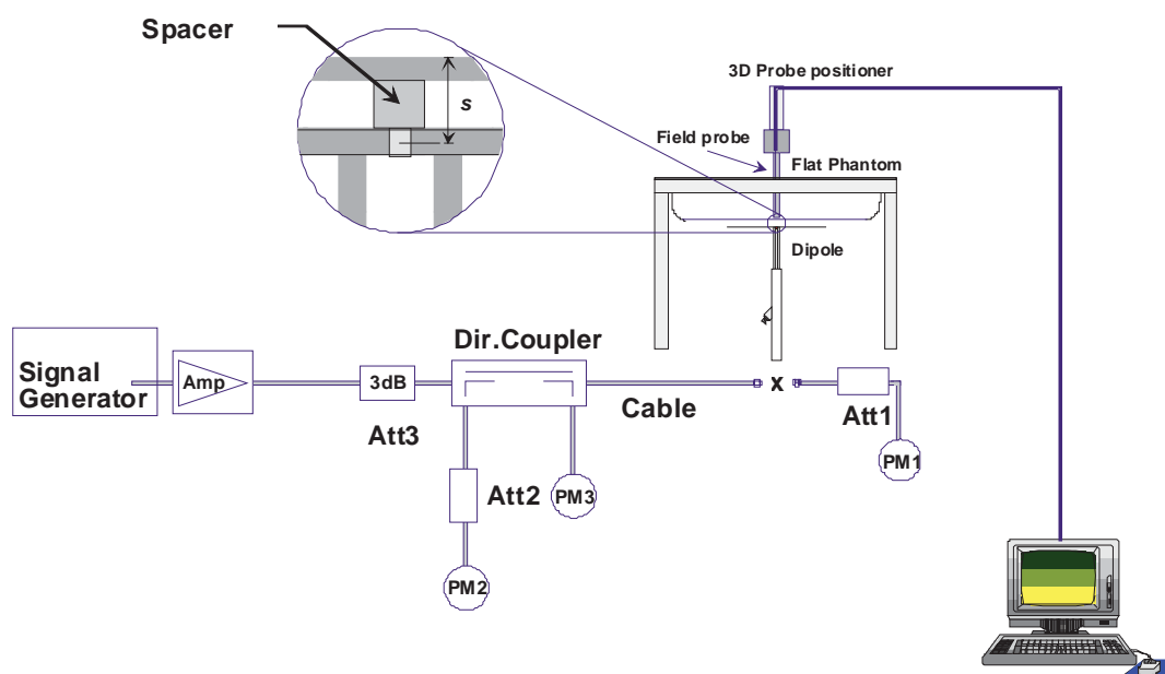
Fig 8.1 System Setup for System Evaluation
