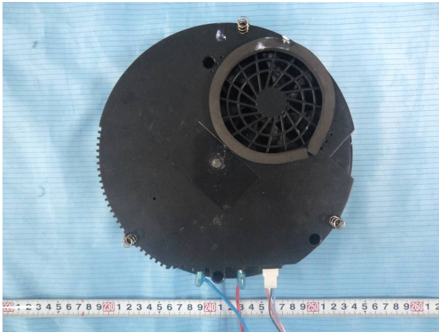
EUT – Right Cover off 1 Back View
