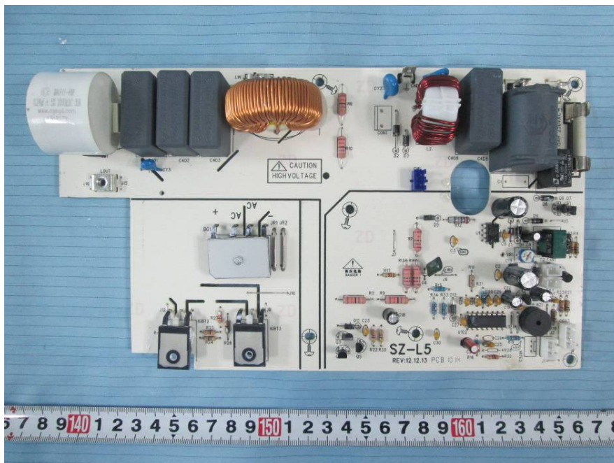
EUT – Uncovered Main Board Top View
