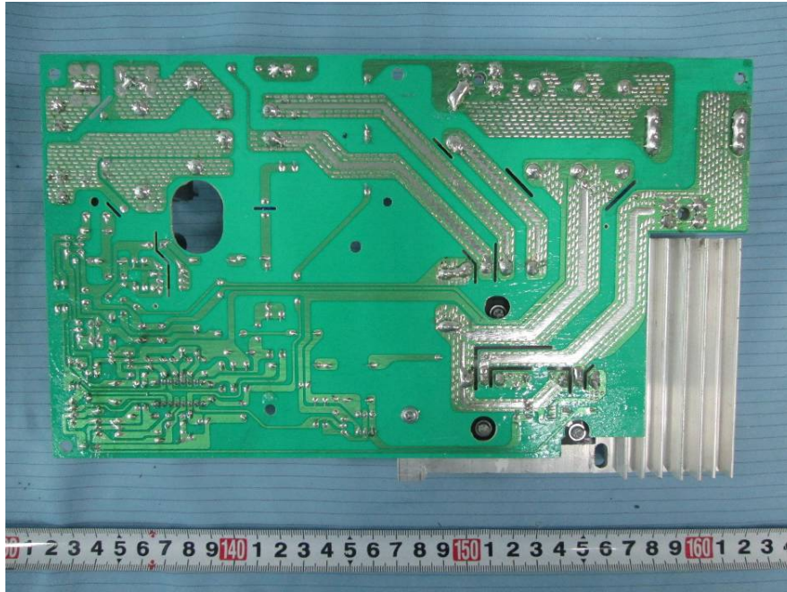
EUT –Cover off Main Board Bottom View
