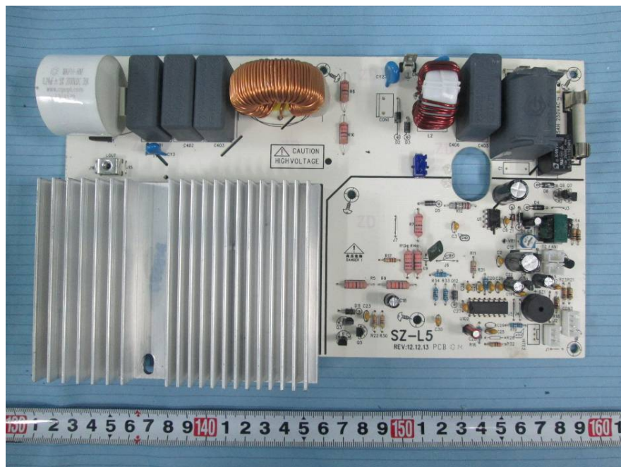
EUT – Cover off Main Board Top View
