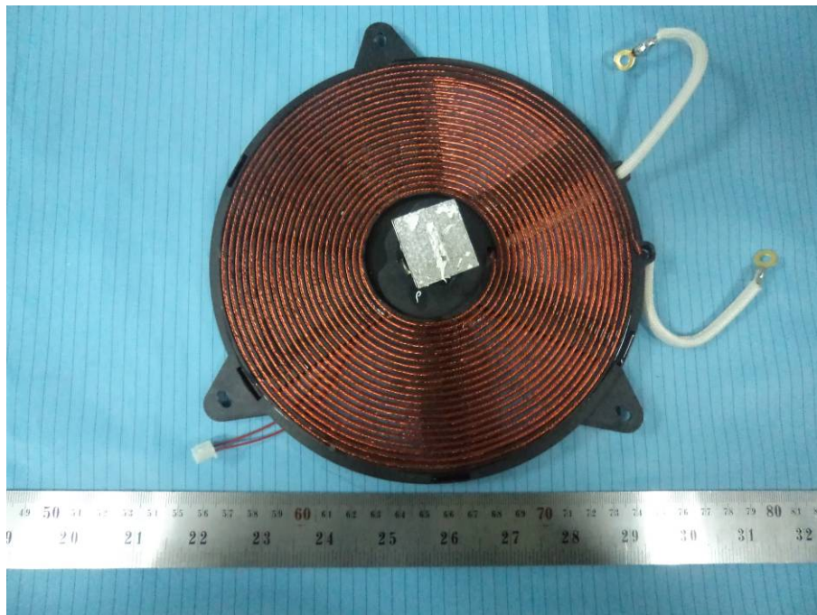
EUT – Coil Top View
