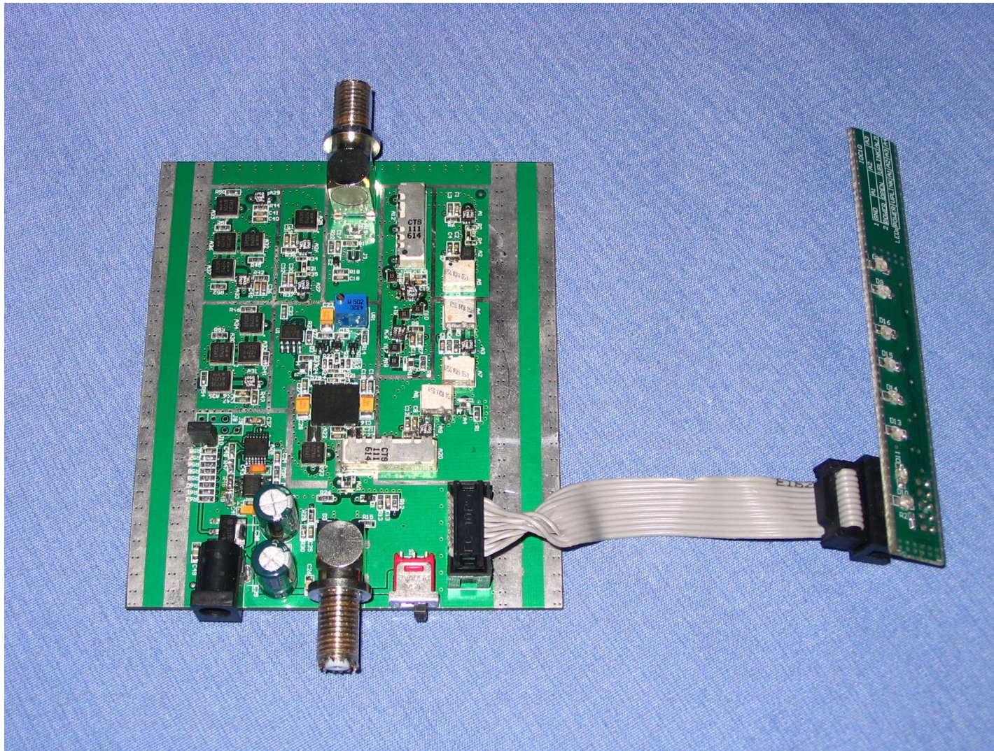
RF Board & Indicator Board
