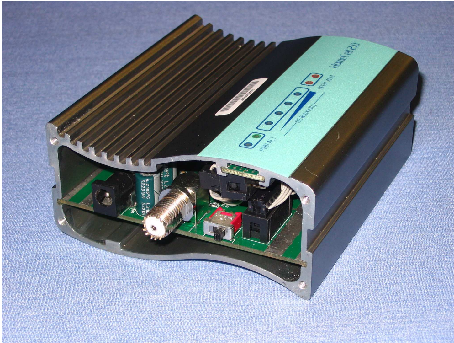
Boards in Chassis/ Left Side
